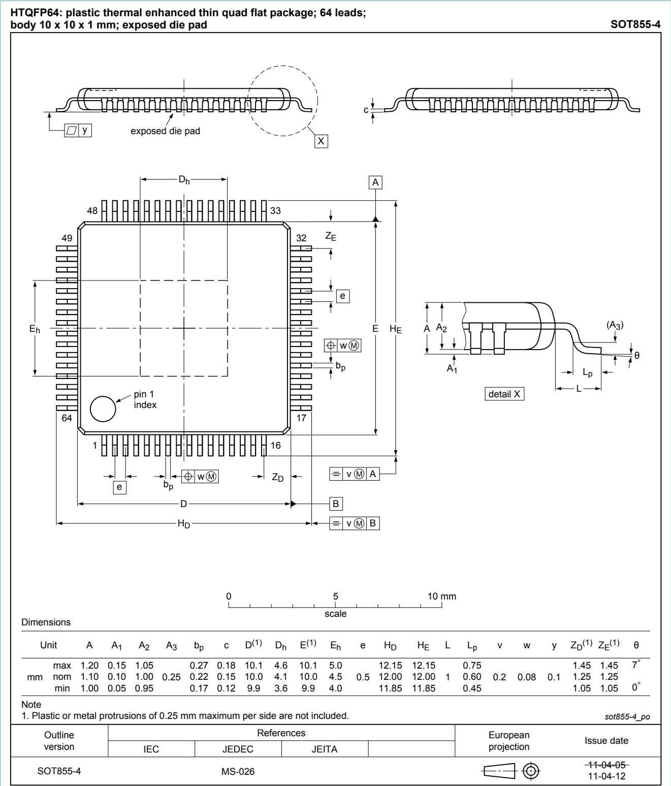
Fig. 1. Package outline HTQFP64 (SOT855-4)
