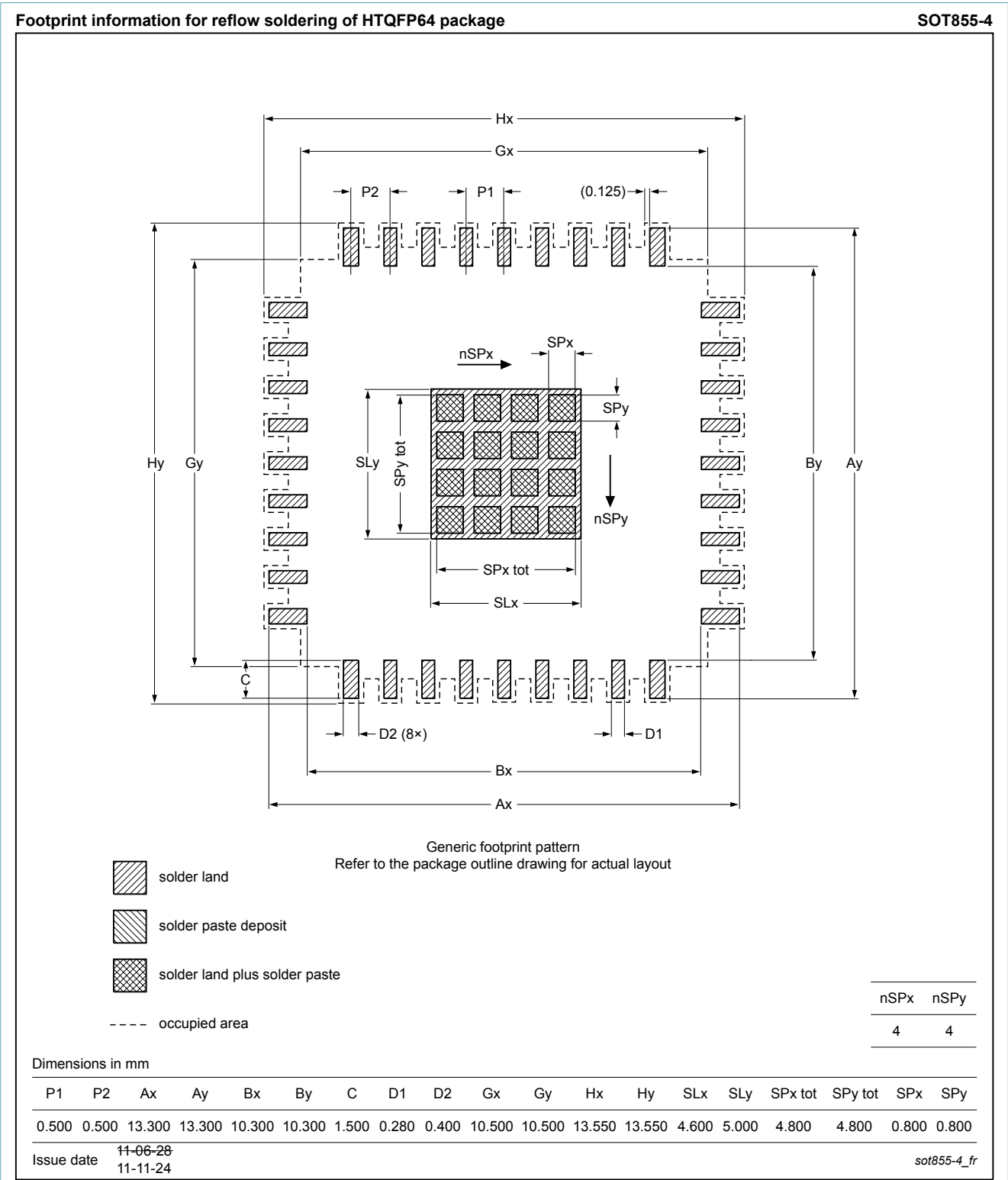
Fig. 2. Reflow soldering footprint for HTQFP64 (SOT855-4)
