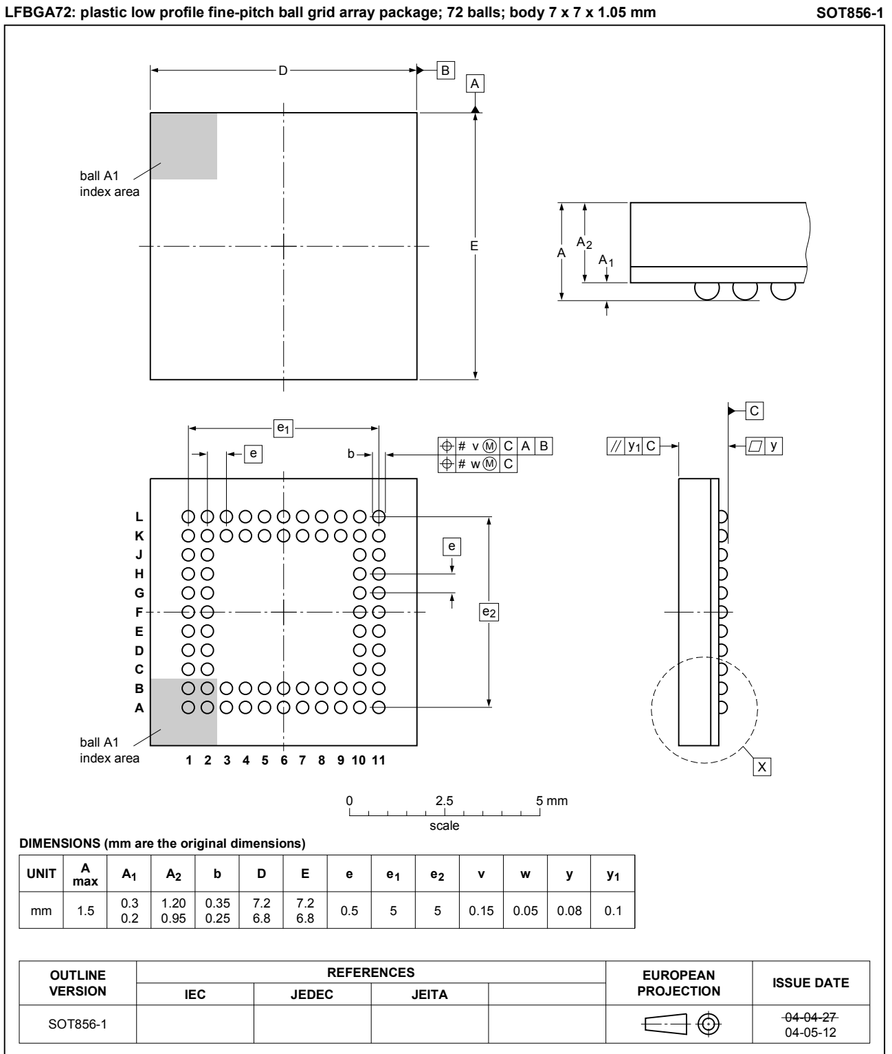
Fig. 1. Package outline LFBGA72 (SOT856-1)
