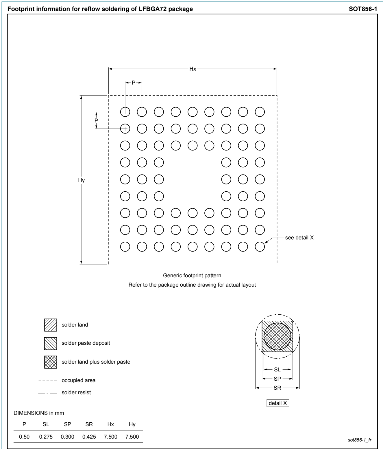
Fig. 2. Reflow soldering footprint for LFBGA72 (SOT856-1)
