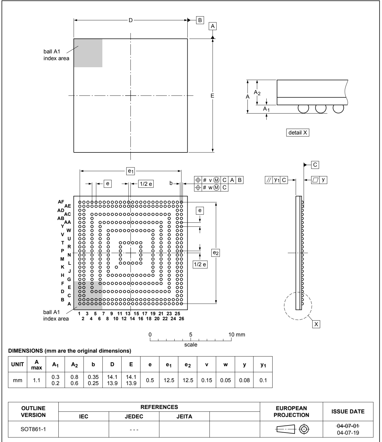
Fig. 1. Package outline TFBGA393 (SOT861-1)
