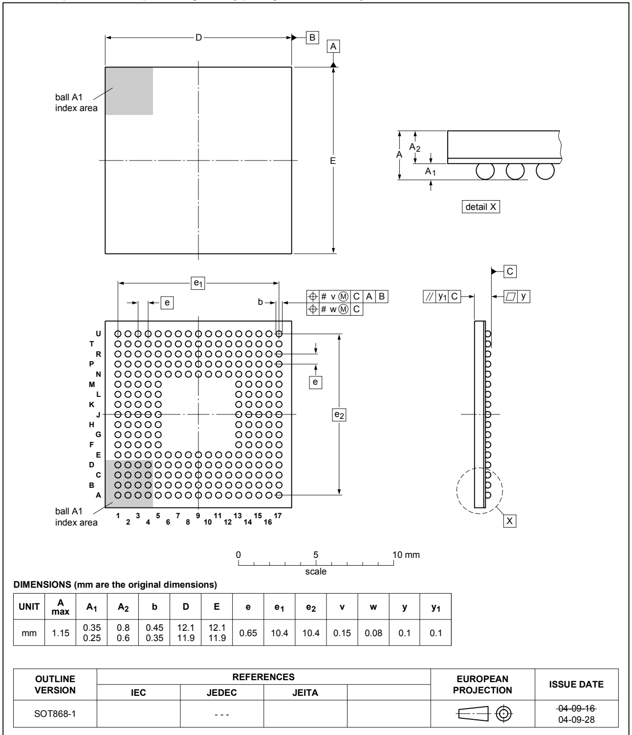
Fig. 1. Package outline TFBGA240 (SOT868-1)
