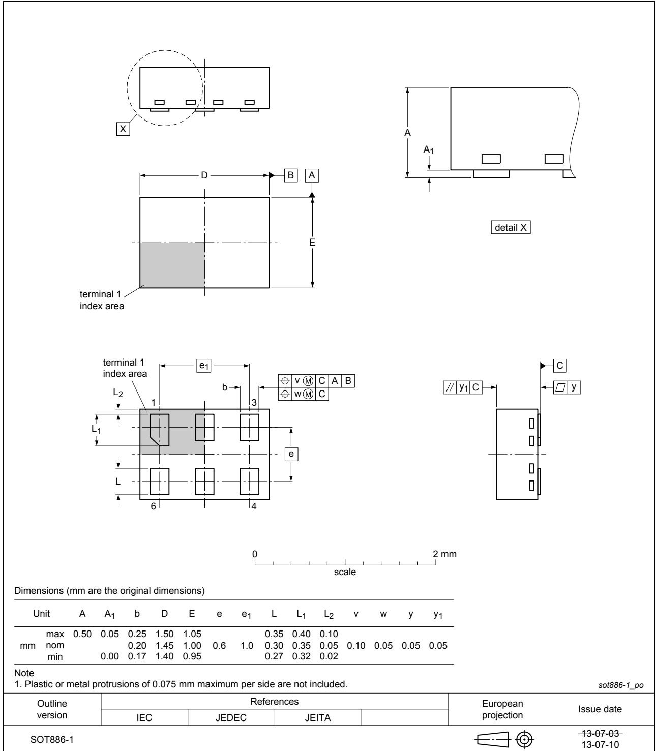
Fig. 1. Package outline XSON6 (SOT886-1)
