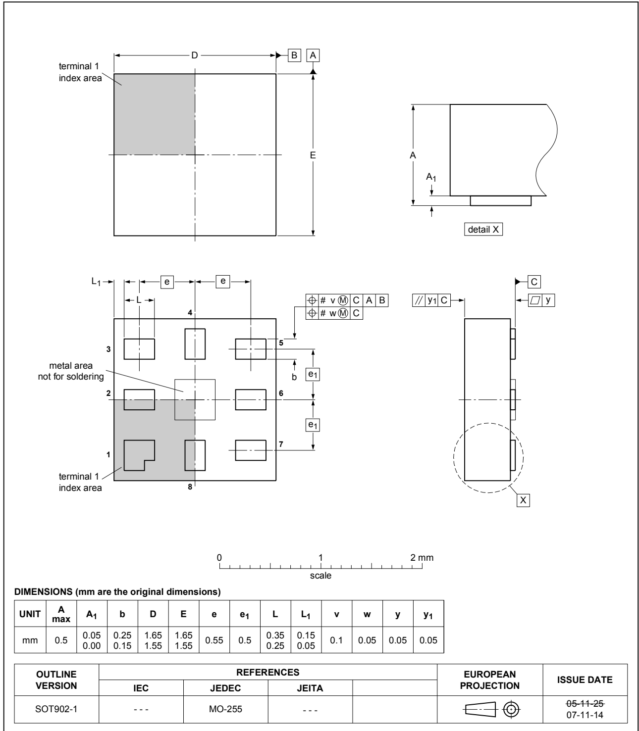
Fig. 1. Package outline XQFN8U (SOT902-1)
