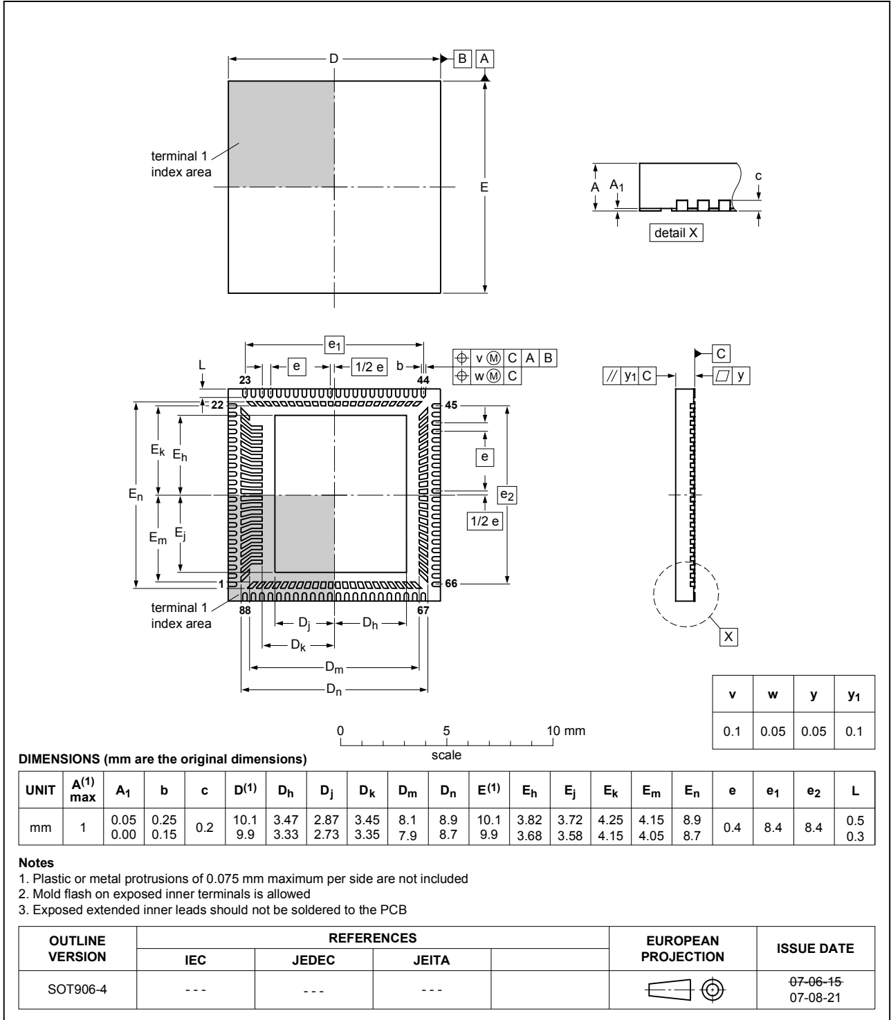
Fig. 1. Package outline HVQFN88 (SOT906-4)
