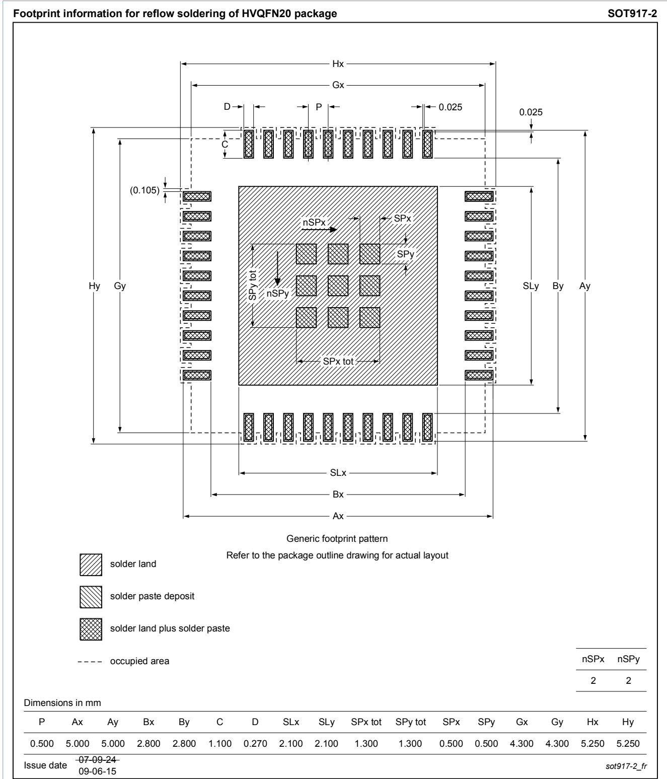
Fig. 1. Reflow soldering footprint for HVQFN20 (SOT917-2)
