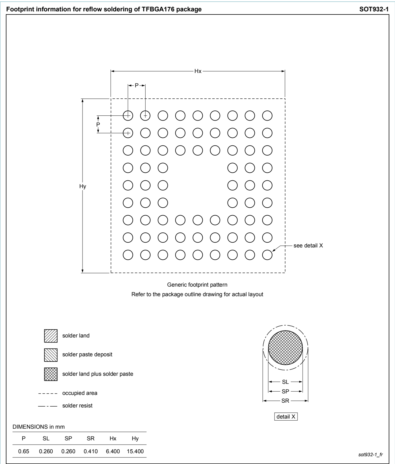
Fig. 2. Reflow soldering footprint for TFBGA176 (SOT932-1)
