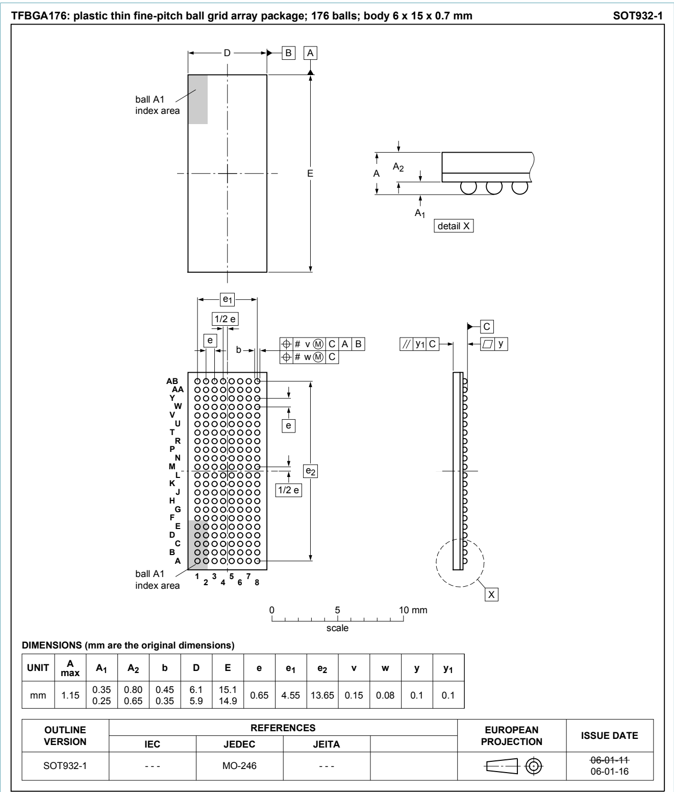
Fig. 1. Package outline TFBGA176 (SOT932-1)
