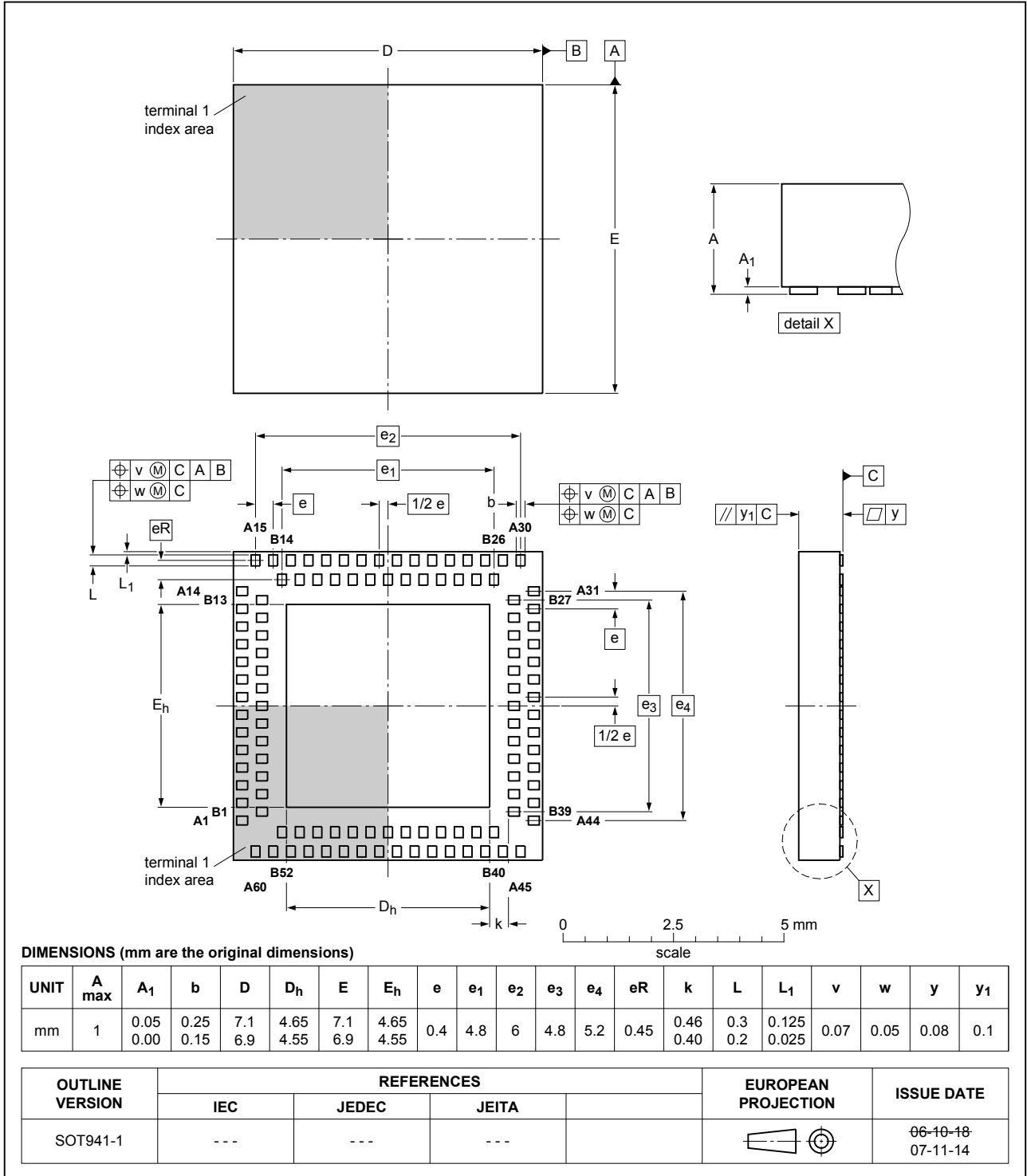
Fig. 1. Package outline HVQFN112U (SOT941-1)
