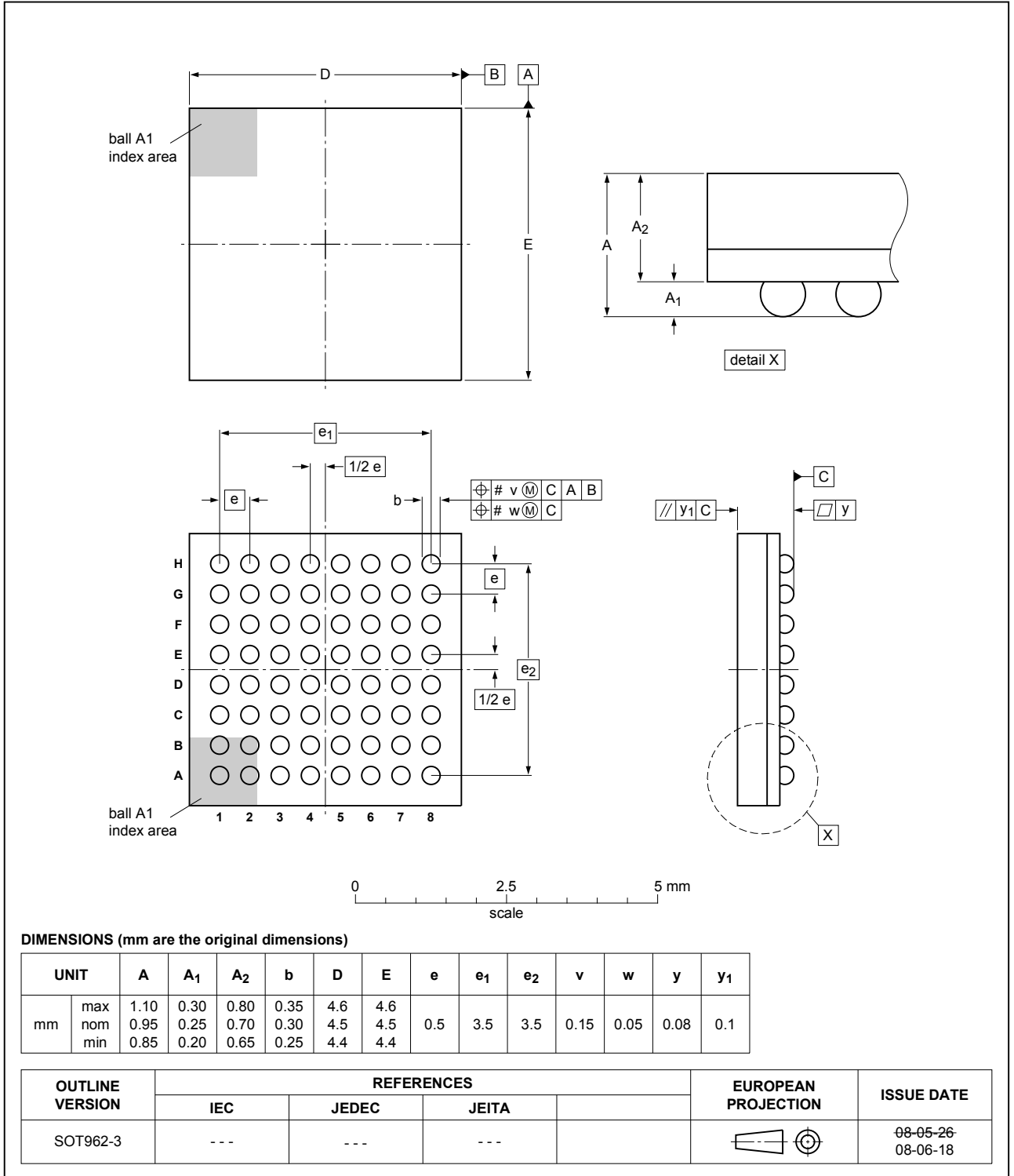
Fig. 1. Package outline TFBGA64 (SOT962-3)
