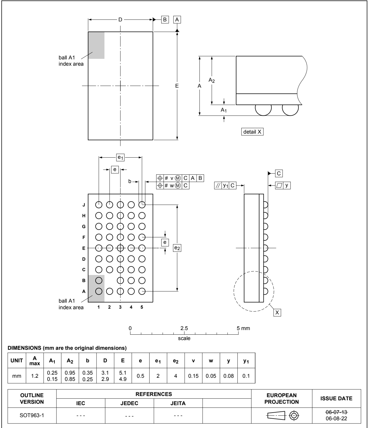
Fig. 1. Package outline TFBGA44 (SOT963-1)
