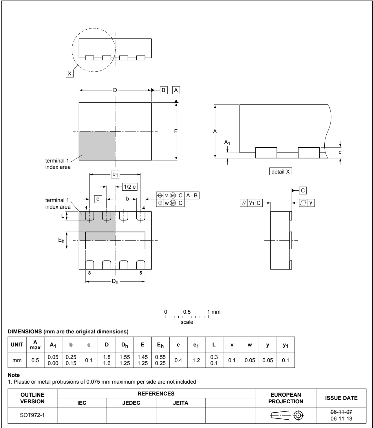
Fig. 1. Package outline HXSON8 (SOT972-1)
