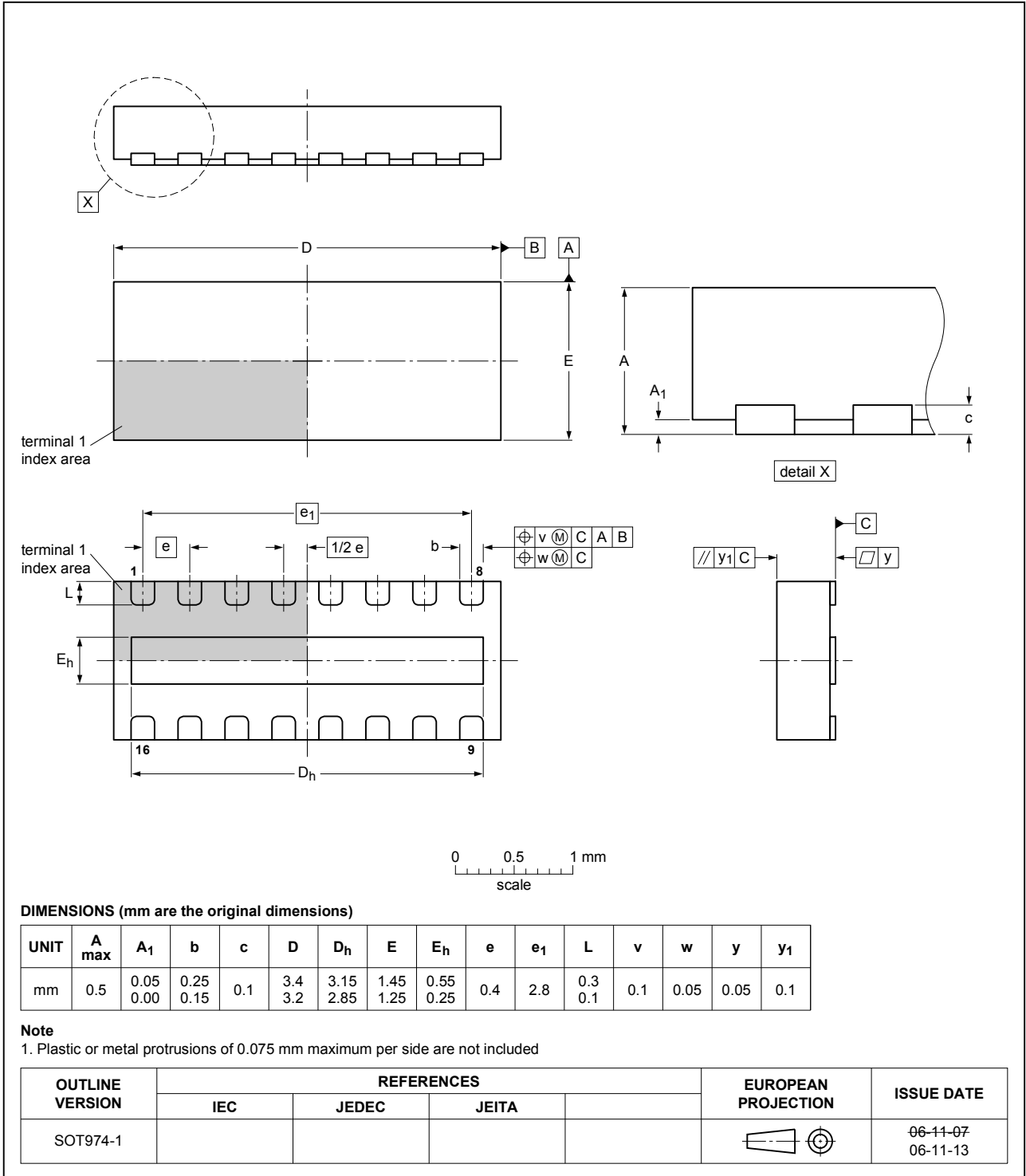
Fig. 1. Package outline HXSON16 (SOT974-1)
