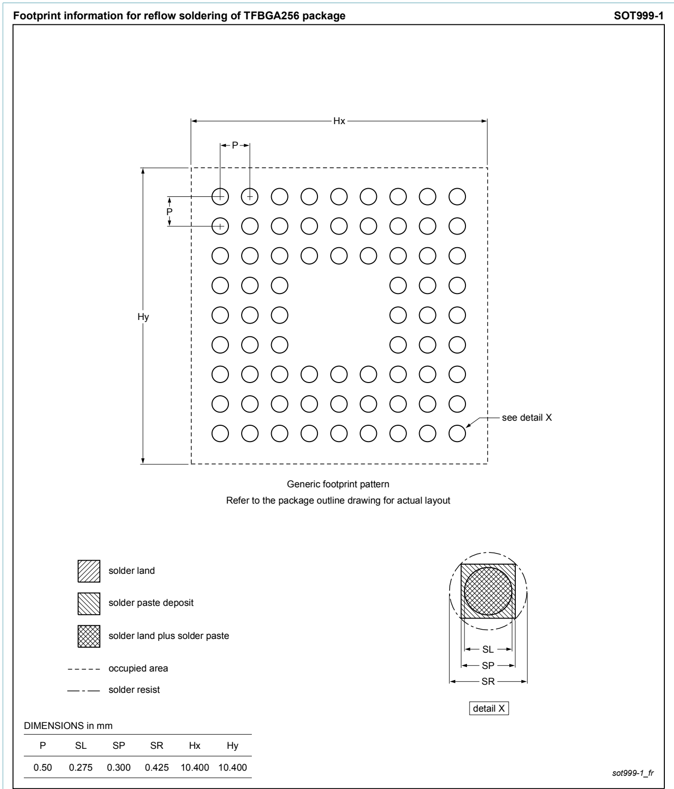
Fig. 2. Reflow soldering footprint for TFBGA256 (SOT999-1)
