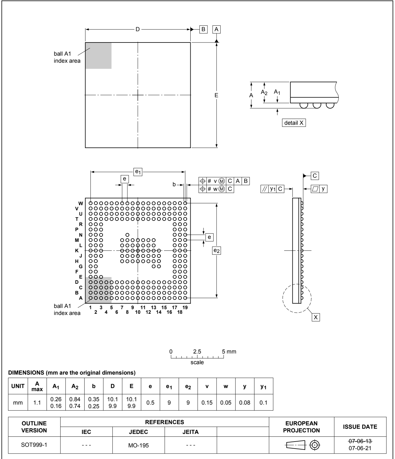
Fig. 1. Package outline TFBGA256 (SOT999-1)
