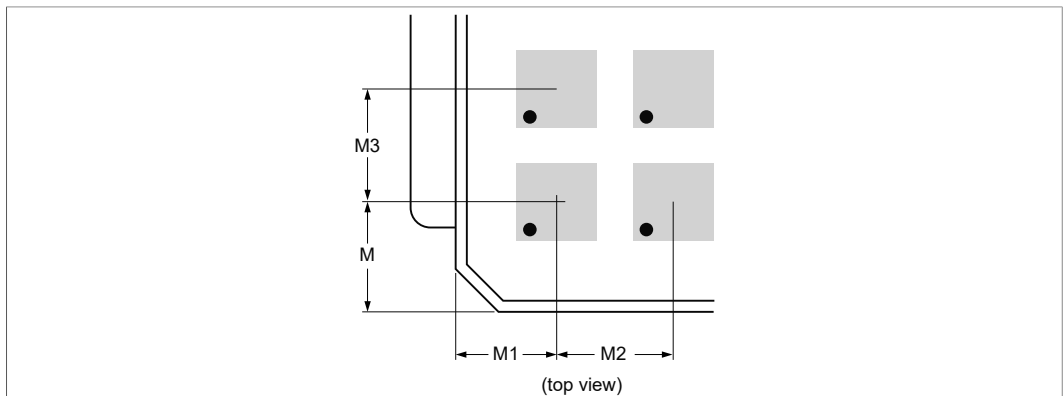
Figure 2. Critical tray dimensions, not drawn to scale
