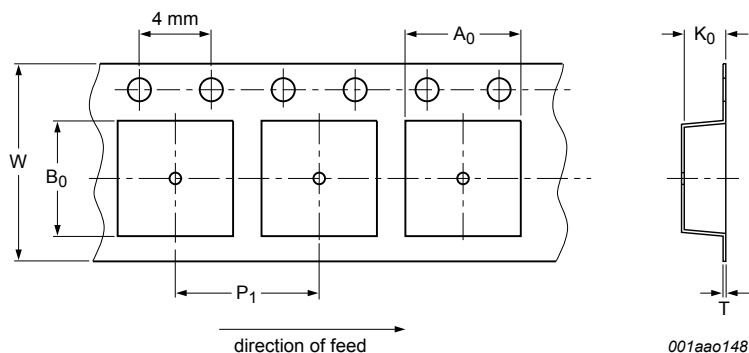
Figure 2. Carrier tape dimensions
