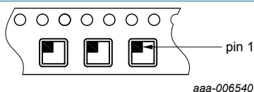
Figure 1. Product orientation in carrier tape
