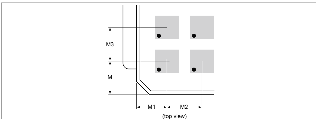
Figure 2. Critical tray dimensions, not drawn to scale
