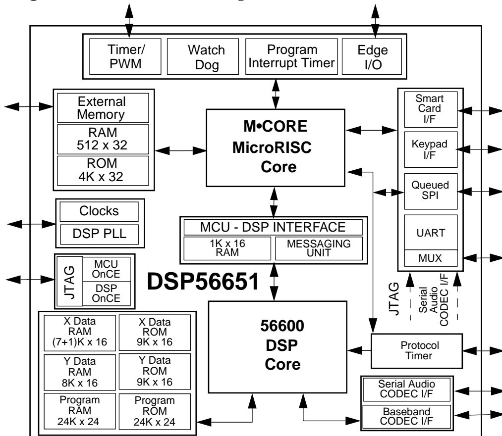
Figure 1 DSP56651 System Block Diagram
