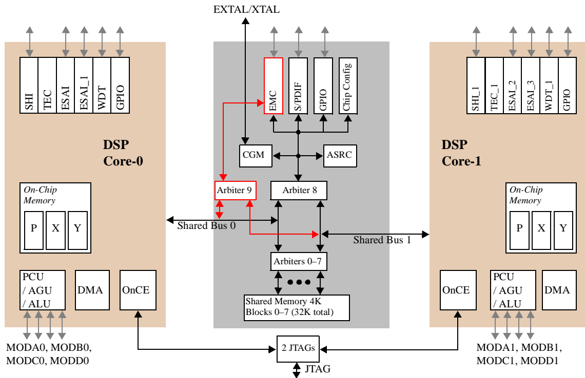
Figure 2. DSP56724 Block Diagram
