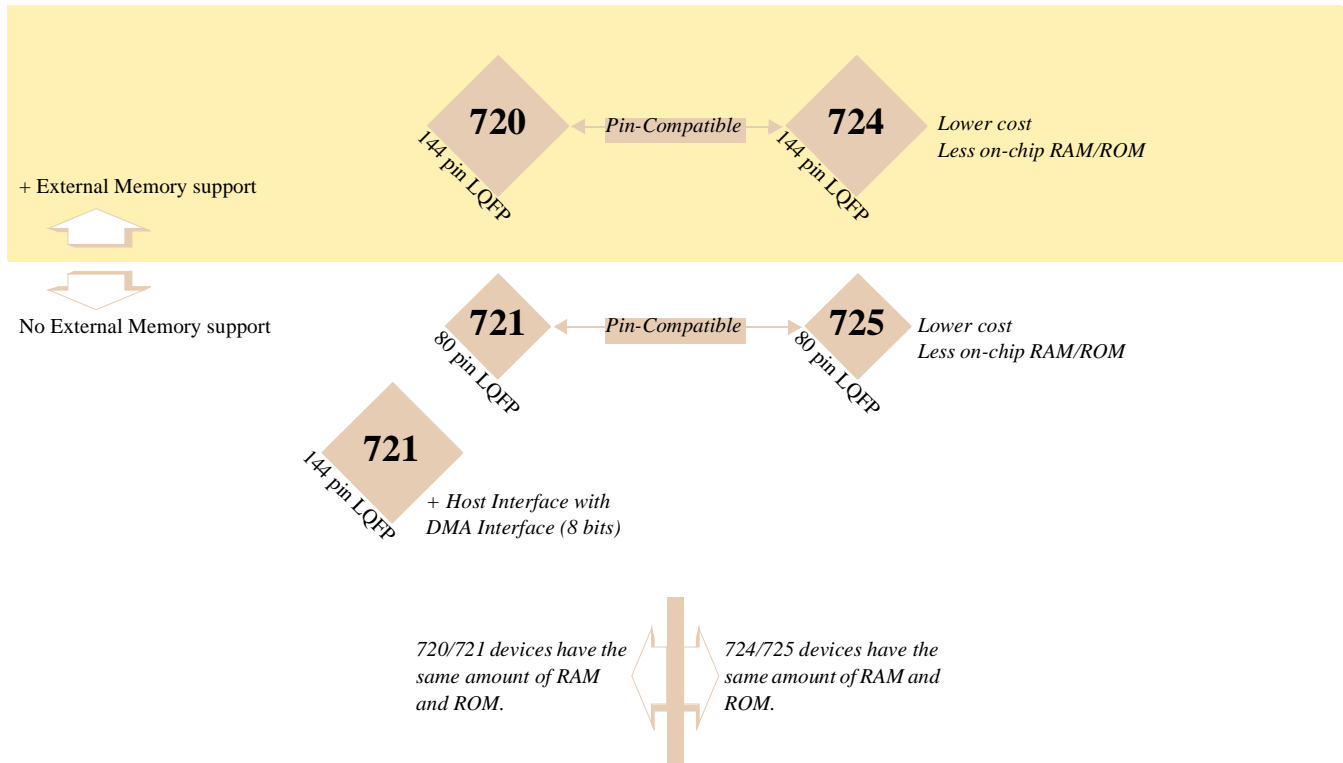
Figure 1. DSP5672x Family
