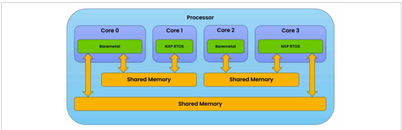
Figure 2. IPCF use case with multiple instances
