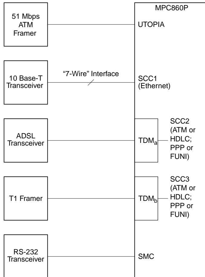
Figure 2. MPC860P System Configuration
