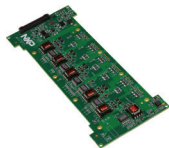
Driver control board (EV-POWERVEVB)
