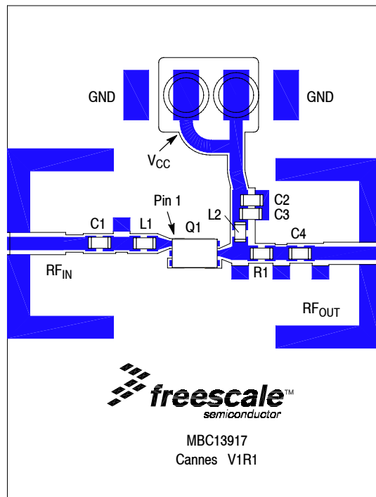
Figure 2. MBC13917 434 MHz Evaluation Circuit Component Layout
