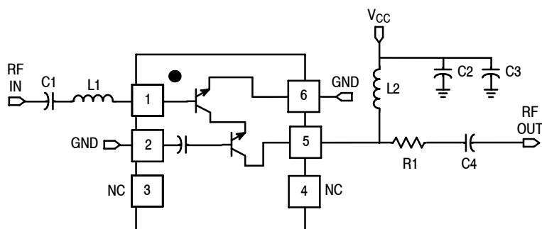
Figure 1. MBC13917 434 MHz Schematic
