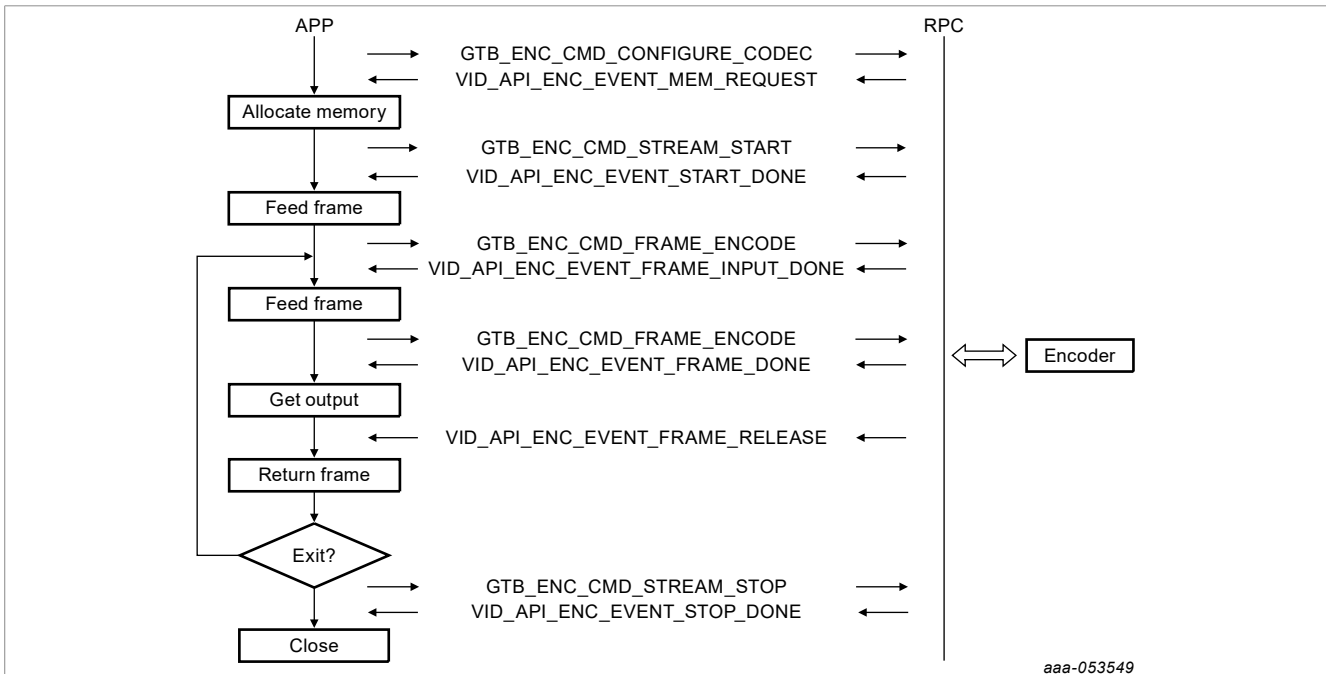
Figure 6. Simple flow for normal encoder
