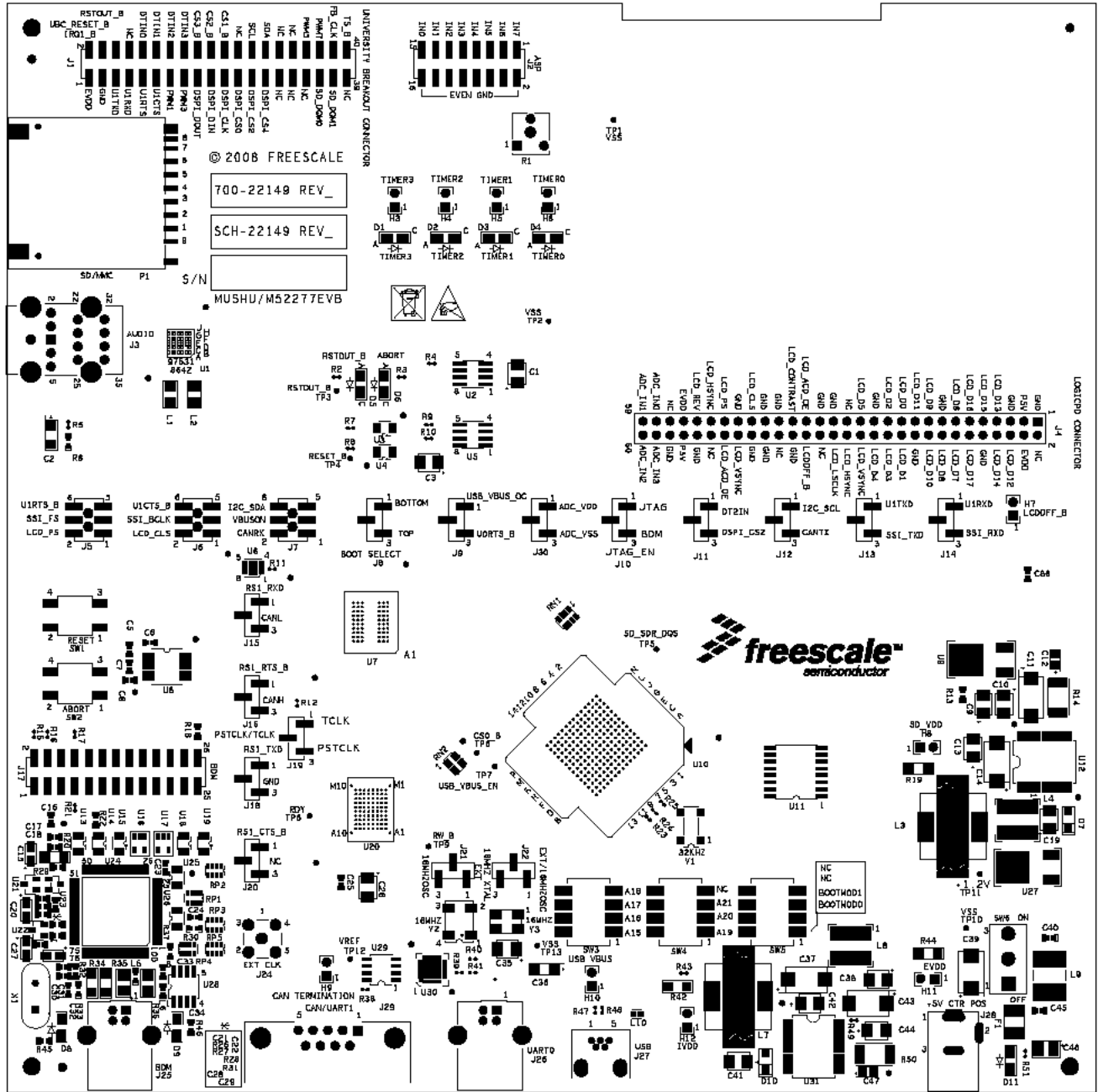
Figure 1. Board Diagram
