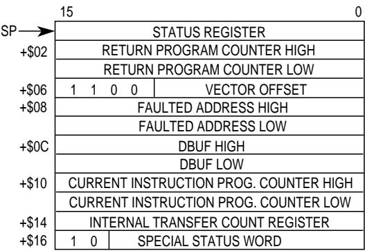
Figure B-15. CPU32 Four- and Six-Word Bus Error Stack Frame, Format $C
