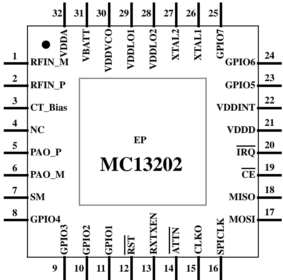
Figure 2-1. MC13202 Pinout
