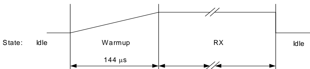
Figure 3-10. RX Timing Profile
