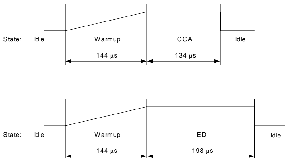
Figure 3-9. CCA and ED Timing Profiles
