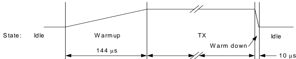
Figure 3-11. TX Timing Profile
