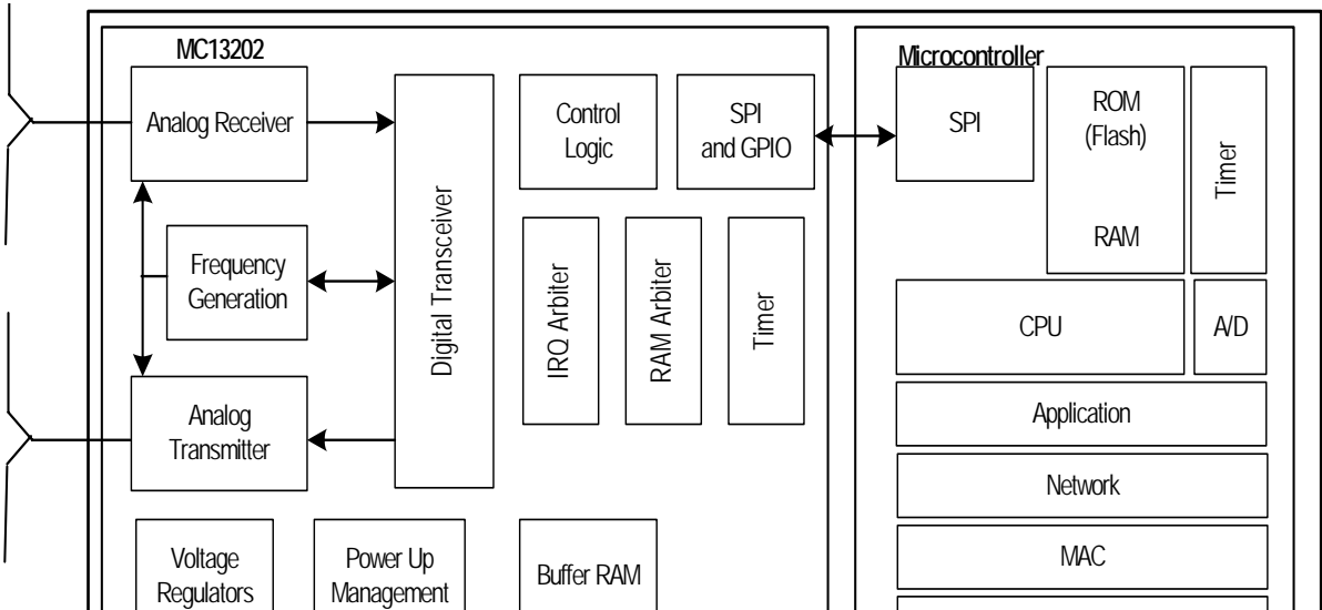
Figure 1-2. System Level Block Diagram
