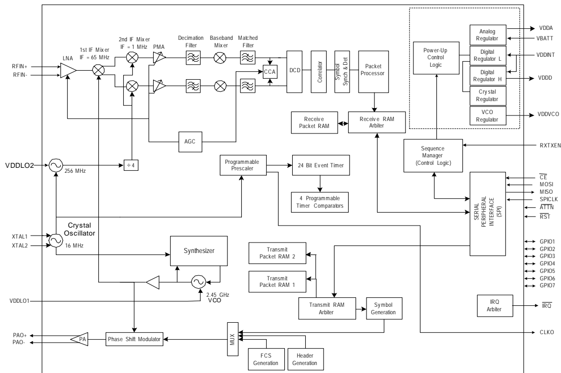
Figure 1-1. MC13202 Simplified Block Diagram
