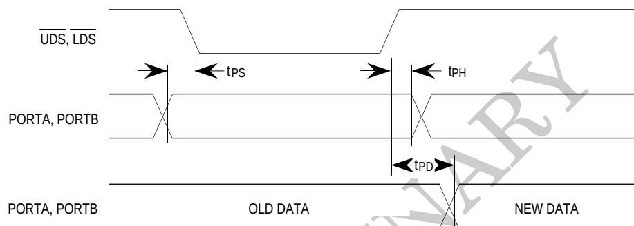
Figure 11-13. Port Timing
