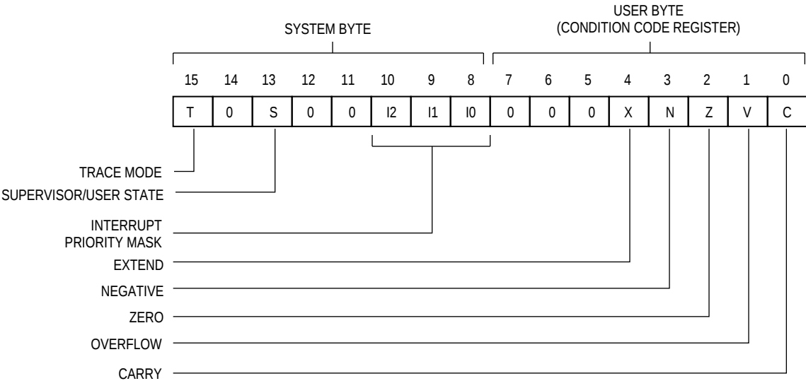
Figure 4-2. Status Register
