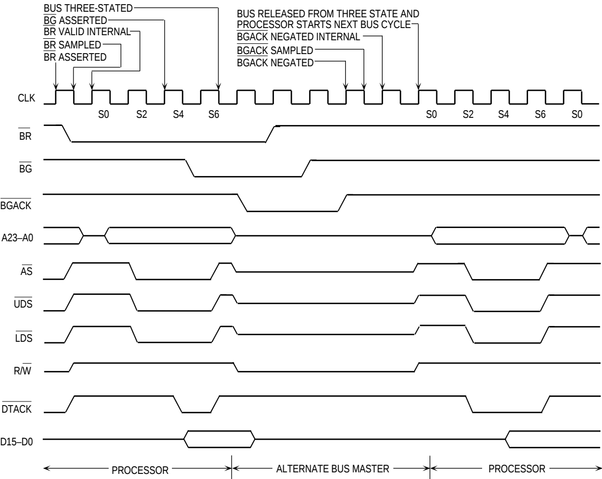
Figure 3-22. Three-Wire Bus Arbitration Timing Diagram—Special Case
