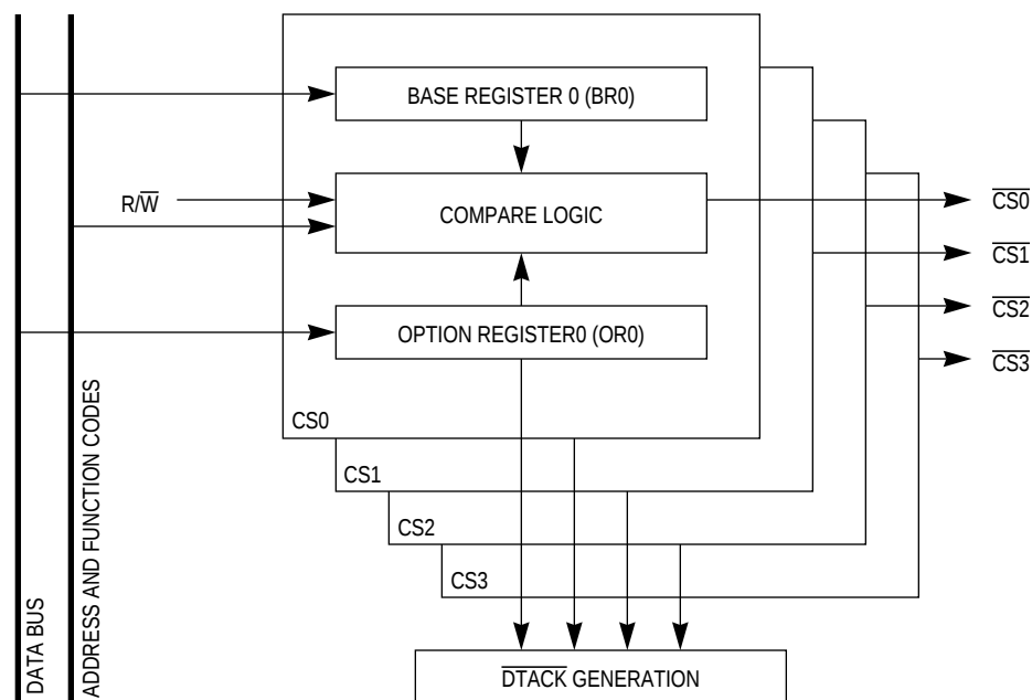
Figure 5-2. Chip-Select Block Diagram
