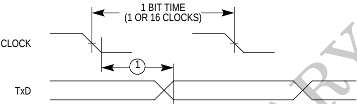
Figure 11-10. Transmitter Timing
