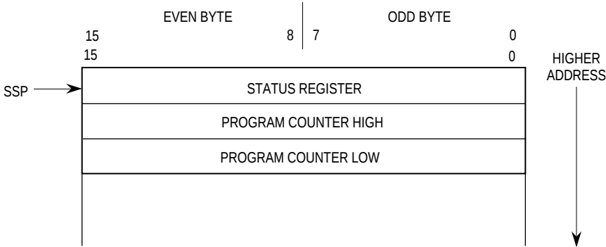
Figure 4-3. General Form of Exception Stack Frame
