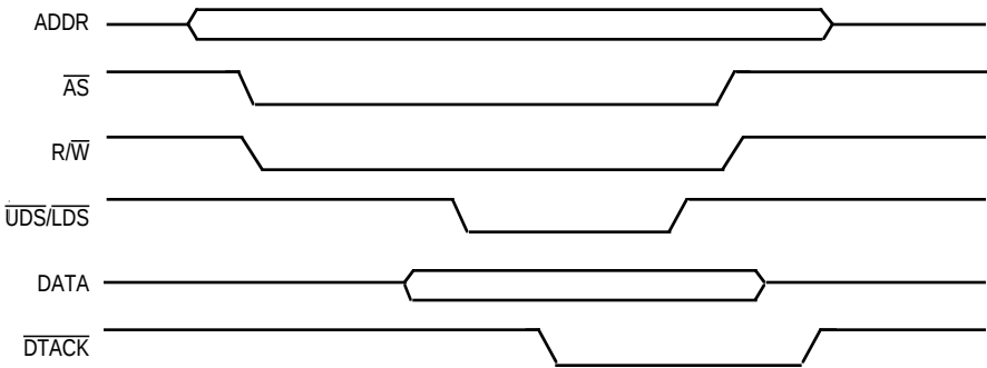
Figure 3-30. Fully Asynchronous Write Cycle
