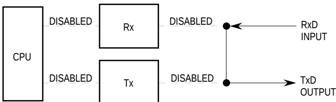
(c) Remote Loopback
