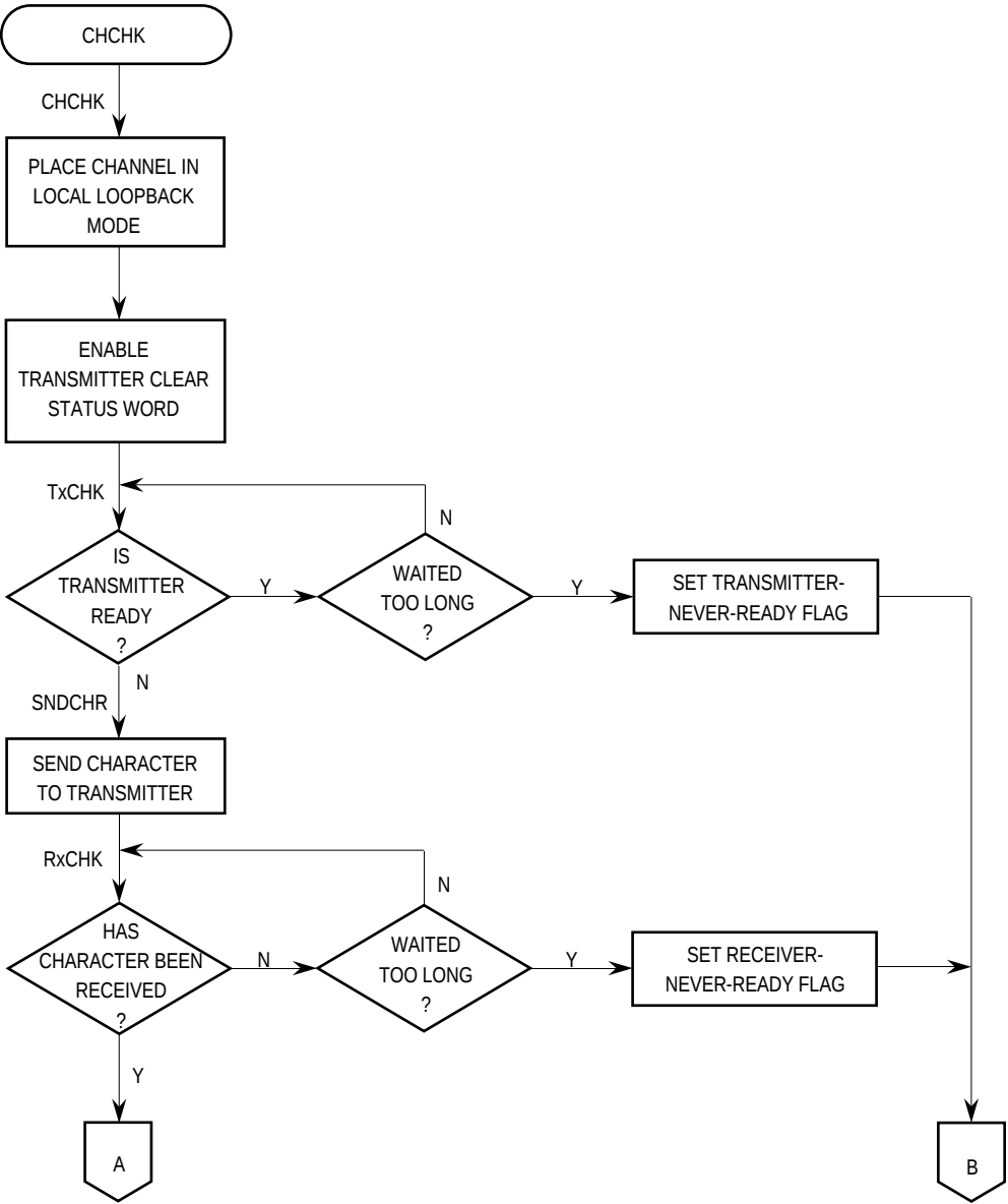
Figure 8-9. Serial Mode Programming Flowchart (2 of 5)
