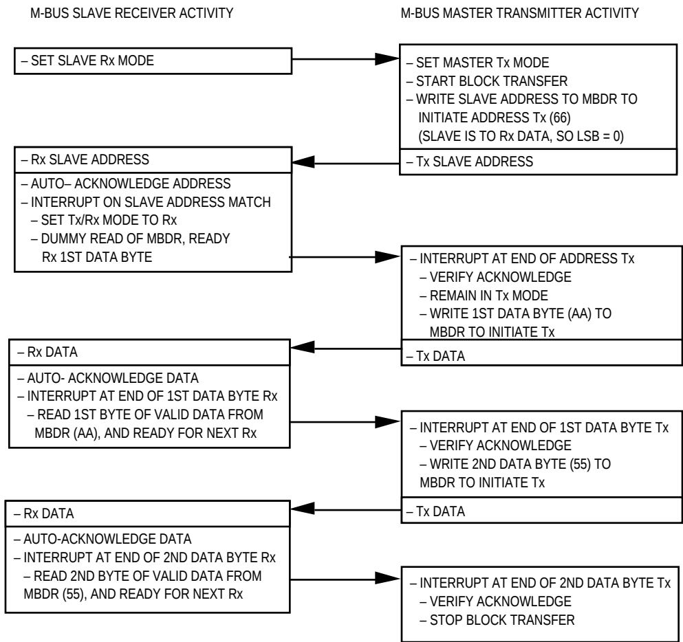
Figure 10-3. Master/Slave Responsibilities for the Master Transmit Block
