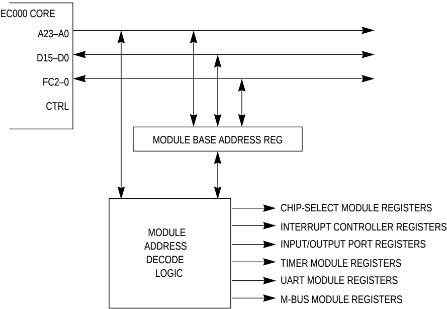
Figure 5-1. Module Base Address, Decode Logic
