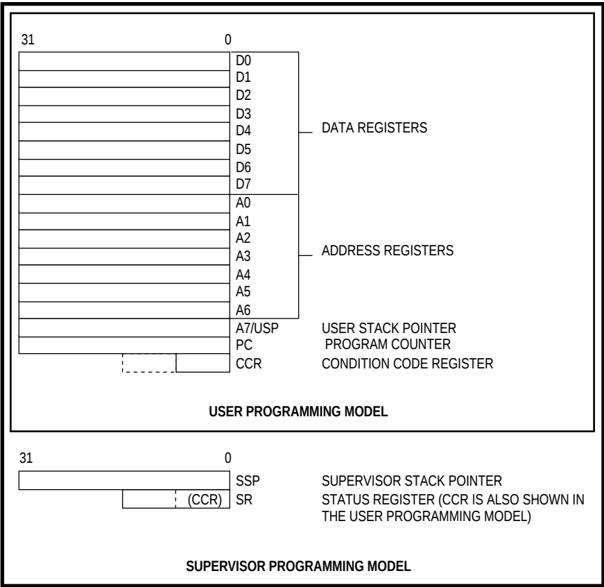
Figure 4-1. Programming Model
