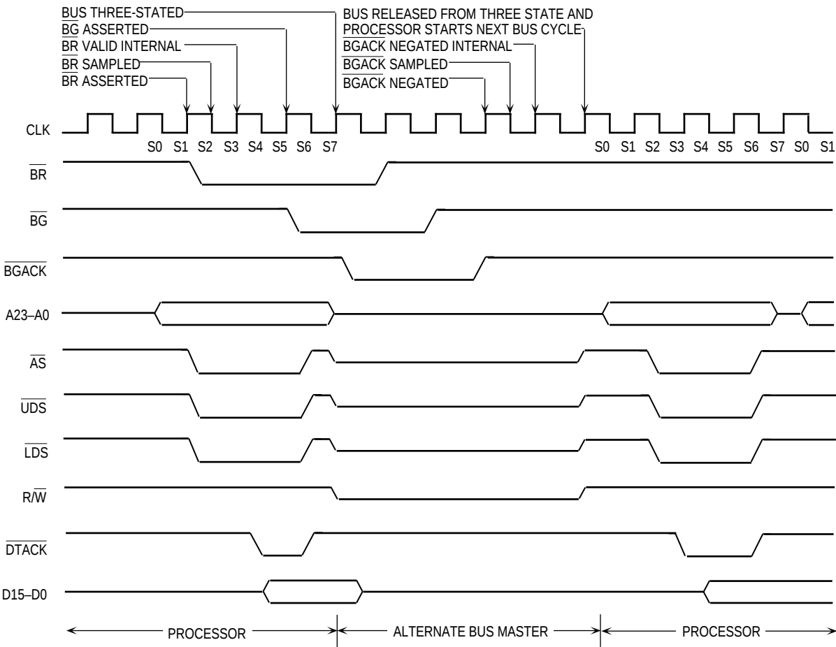
Figure 3-20. Three-Wire Bus Arbitration Timing Diagram—Processor Active
