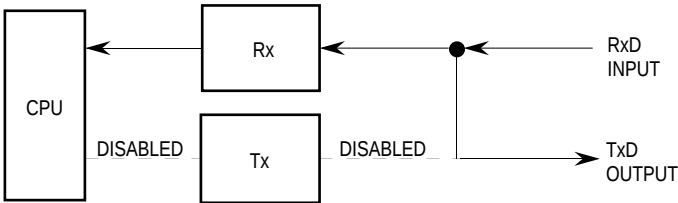
(a) Automatic Echo
