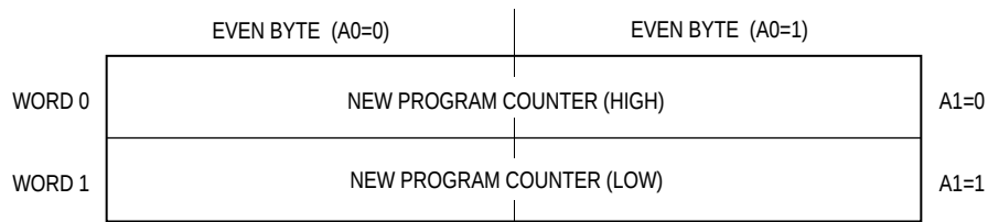
Figure 4-5. Exception Vector Format
