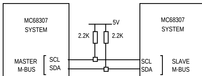
Figure 10-2. Hardware Setup
