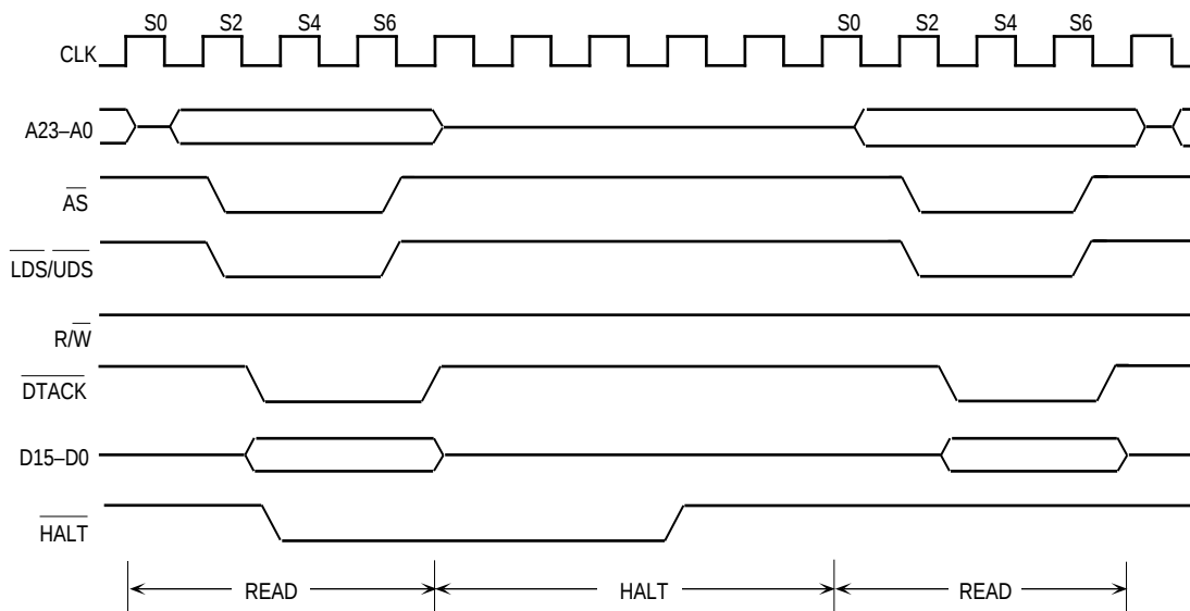
Figure 3-28. Halt Operation Timing Diagram
