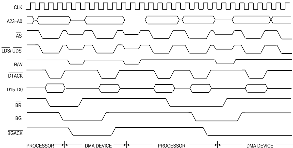
Figure 3-16. Three-Wire Bus Arbitration Timing Diagram
