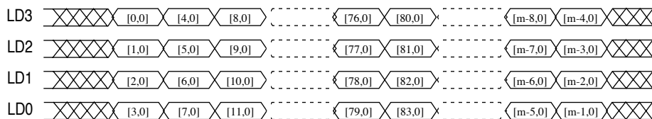
4-BIT LCD DATA BUS (PBSIZ = 10)
