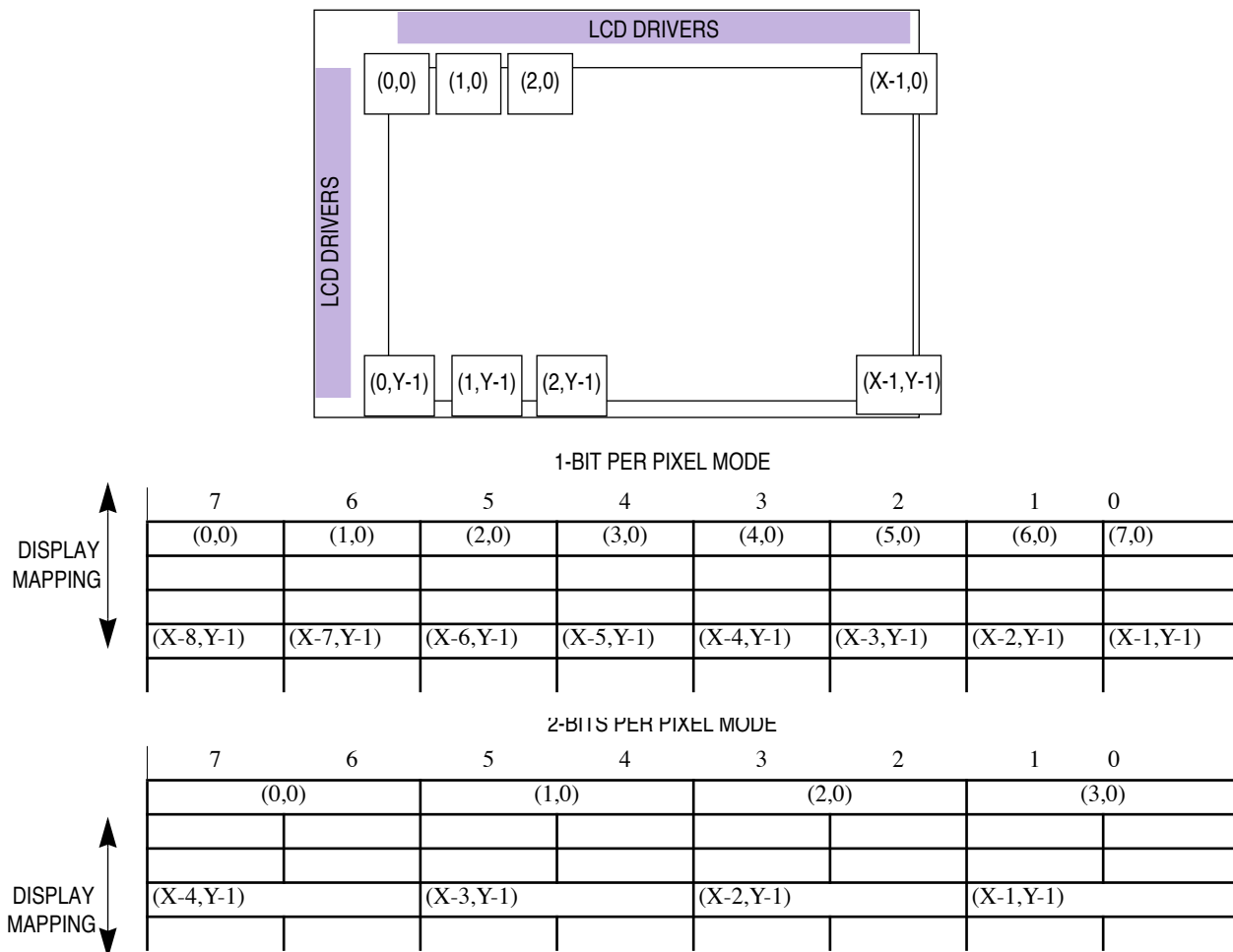
Figure 12-4. Mapping Memory Data on the Screen
