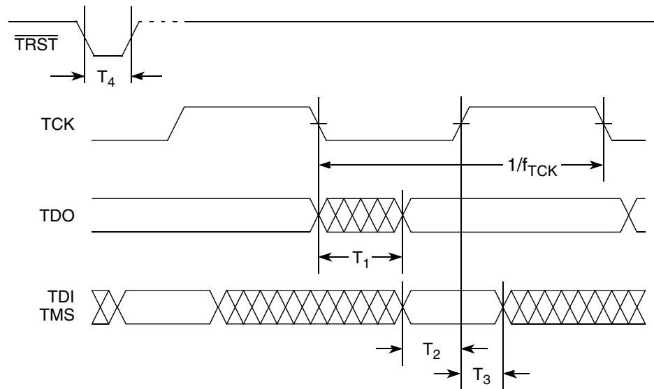
Figure 7-11. JTAG I/O Timing Diagram
