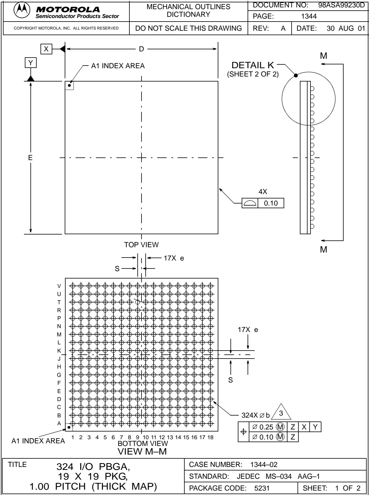
Figure 7-1. 324 MAPBGA Nomenclature
