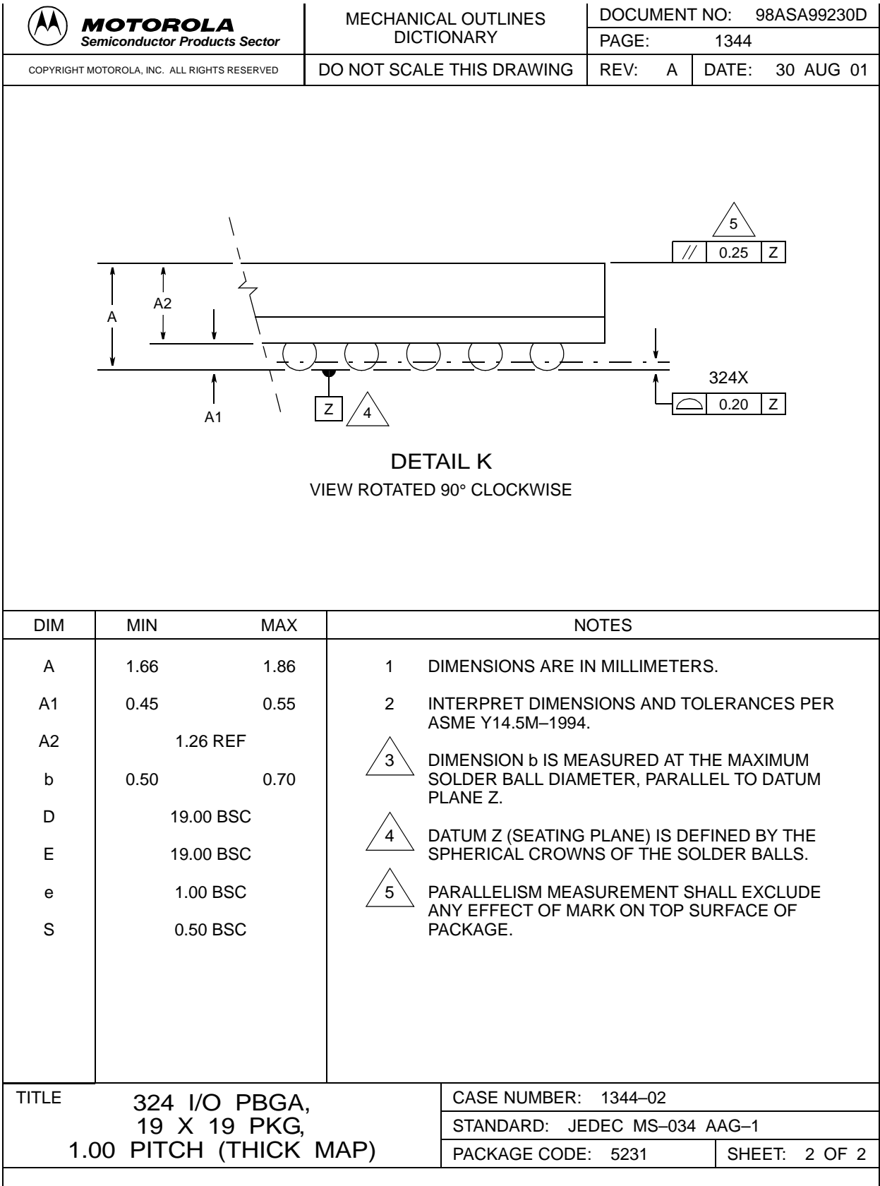
Figure 7-2. MAPBGA Dimensions
