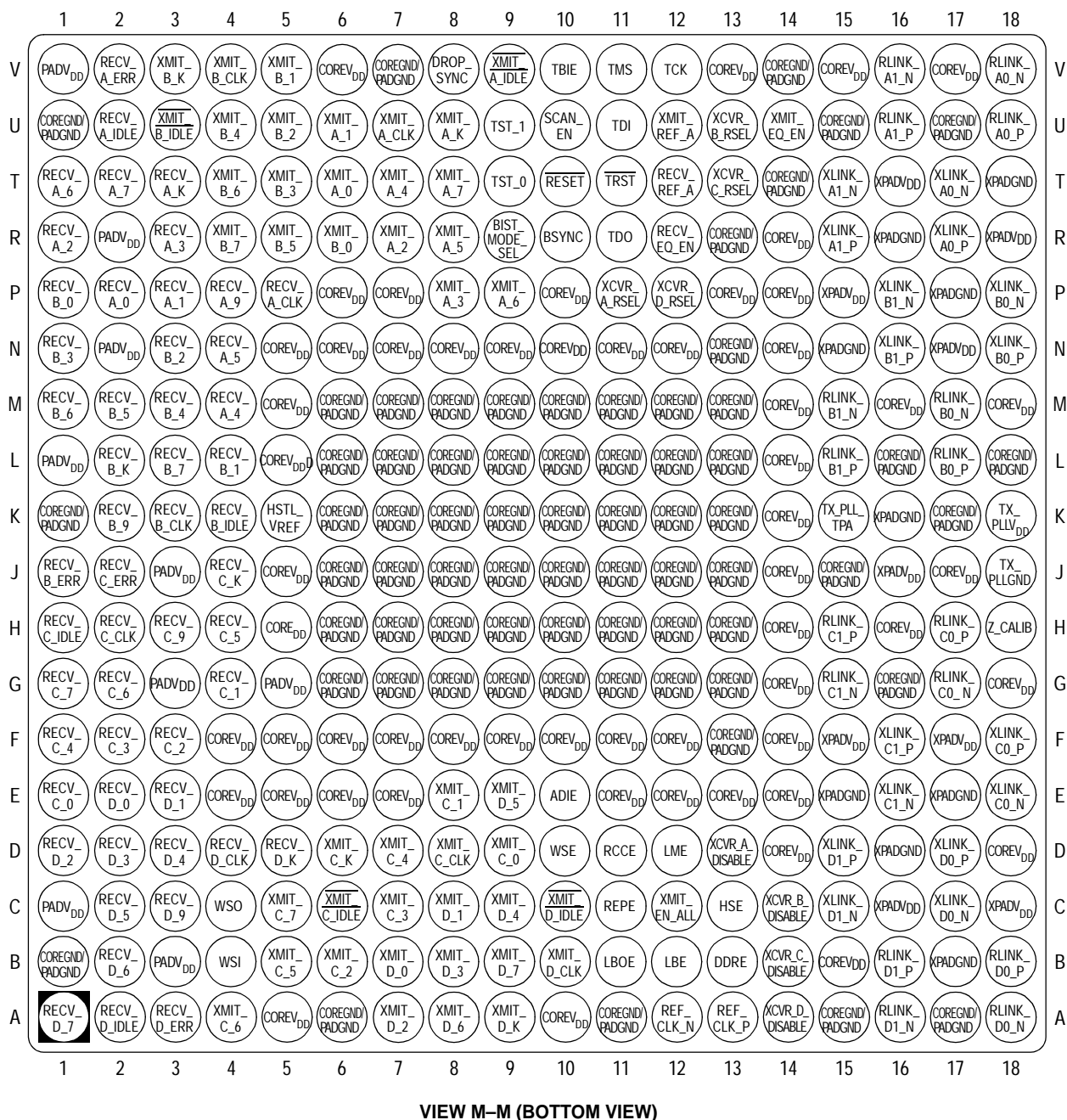
Figure 7-3. 324 MAPBGA Package
