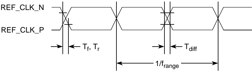
Figure 6-6. Reference Clock Timing Diagram
