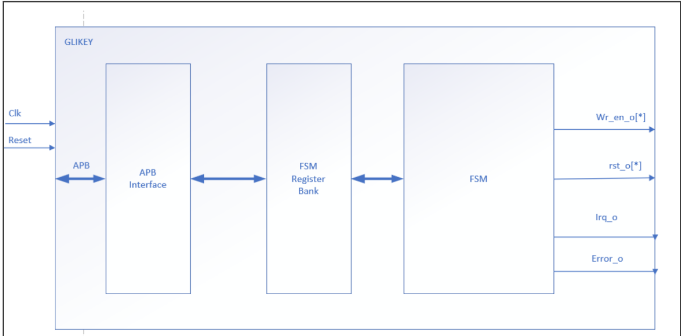
Figure 44. GLIKEY Block Diagram
