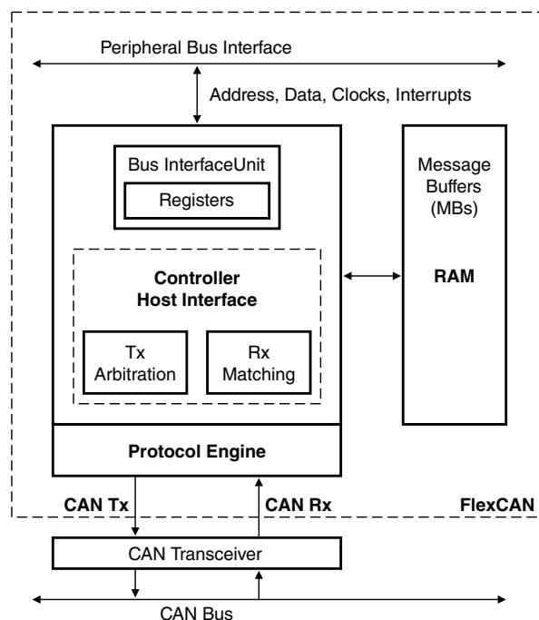
Figure 49-1. FlexCAN block diagram
