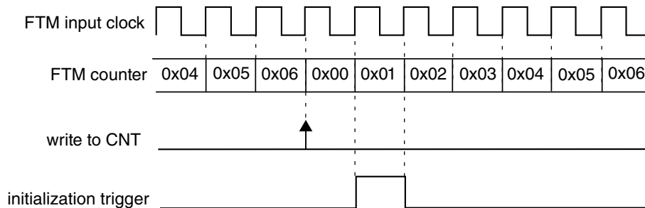
Figure 41-89. Example of the generation of the initialization trigger in the case 2.
