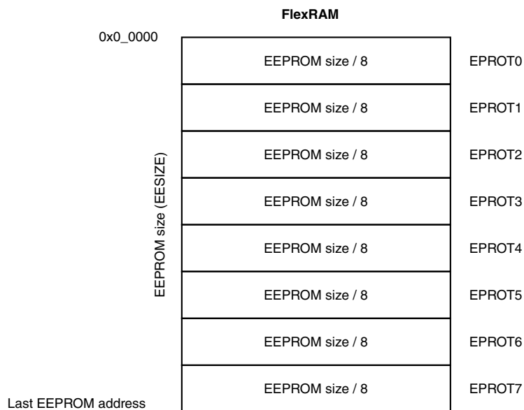
Figure 32-8. EEPROM protection
