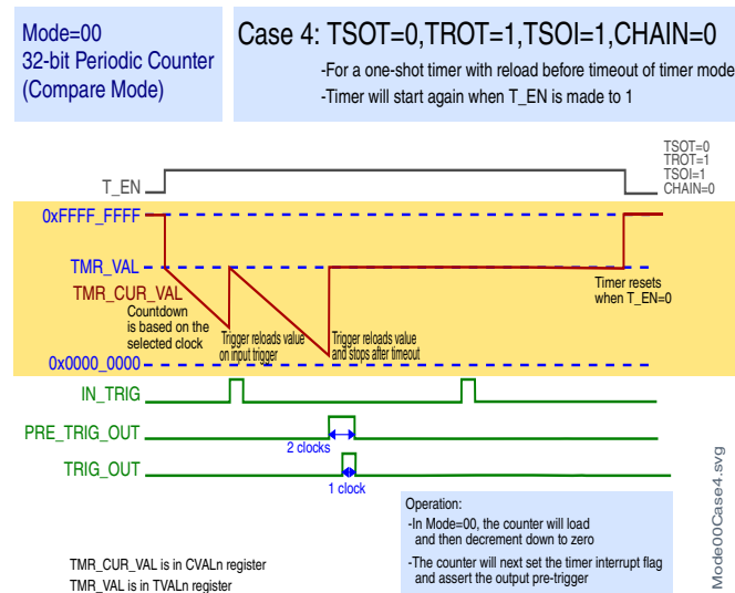
Figure 42-8. Case 4: TSOT = 0, TROT = 1, TSOI = 1, CHAIN = 0
