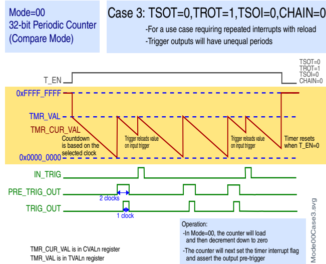
Figure 42-7. Case 3: TSOT = 0, TROT = 1, TSOI = 0, CHAIN = 0
