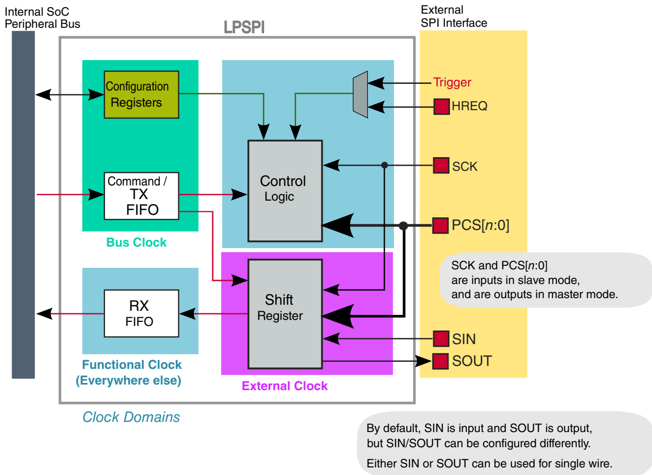
Figure 45-1. Block Diagram
