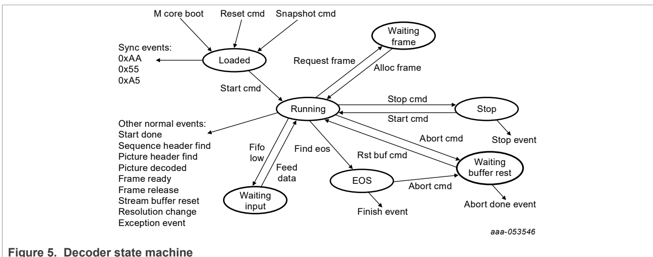
Figure 5. Decoder state machine
