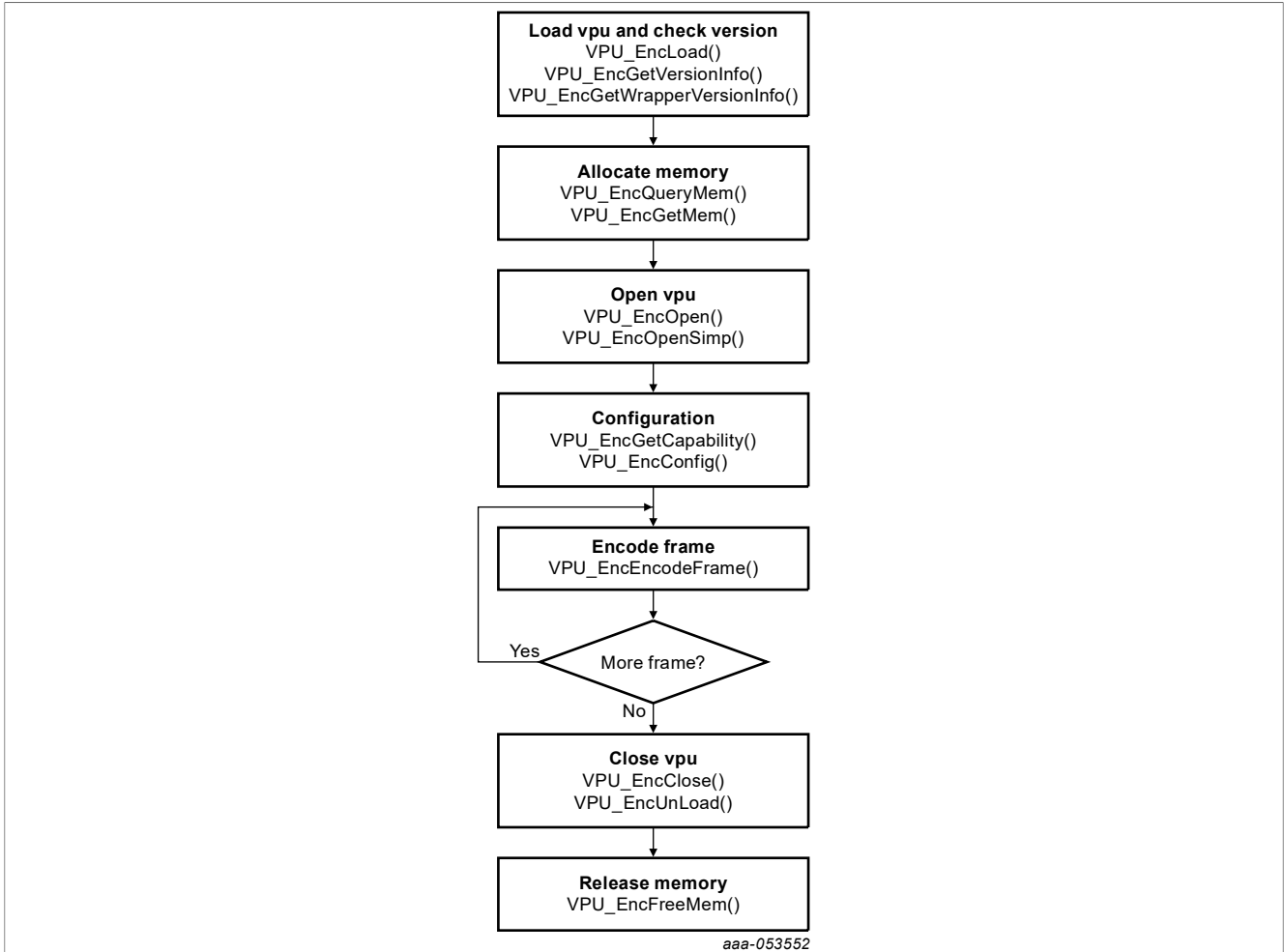
Figure 3. Typical encoding process
