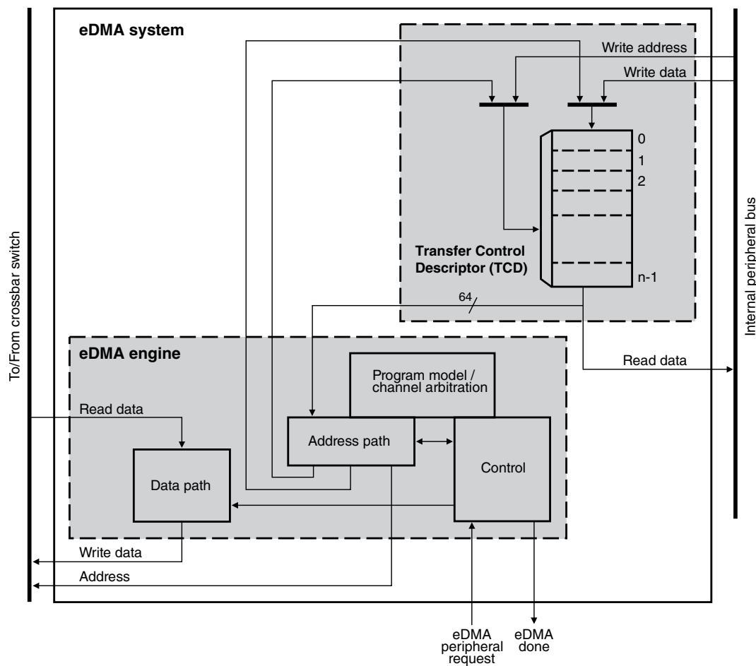
Figure 11-1. Block diagram
