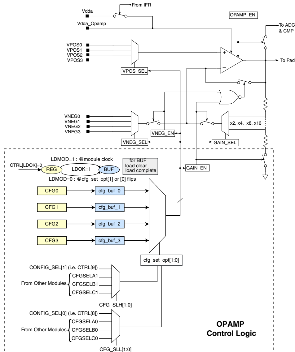
Figure 25-1. OPAMP block diagram
