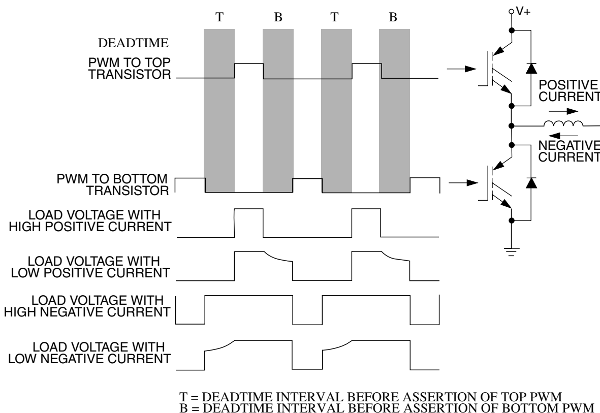
Figure 26-24. Output voltage waveforms
