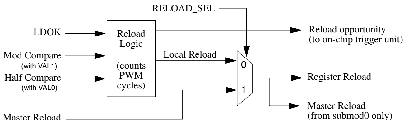
Figure 26-14. Register reload logic of 1 submodule
