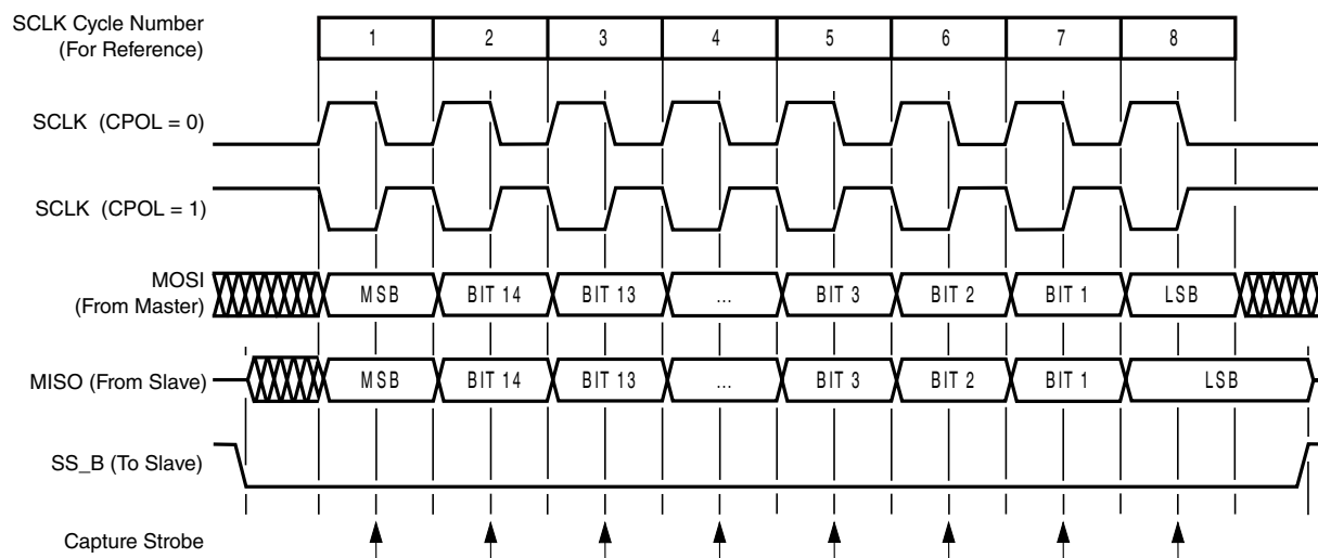
Figure 30-7. Transaction Format ( \text{CPHA} = 1 )
