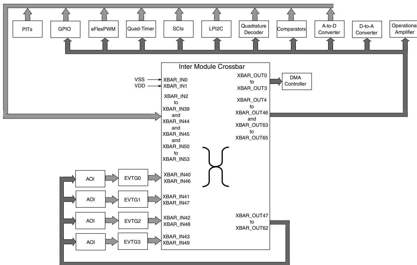
Figure 15-1. XBAR inter-connection
