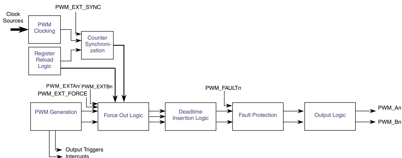
Figure 26-13. High-level output PWM generation block diagram
