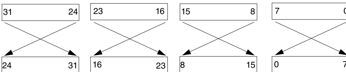
Figure 21-2. Transpose type 01
