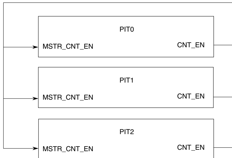
Figure 28-3. CNT_EN Connection Between Multiple PITs
