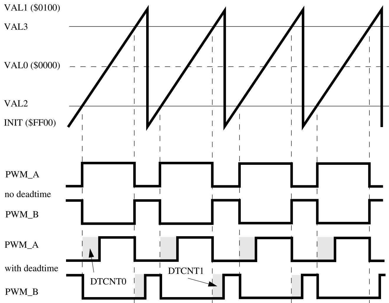
Figure 26-21. Deadtime insertion
