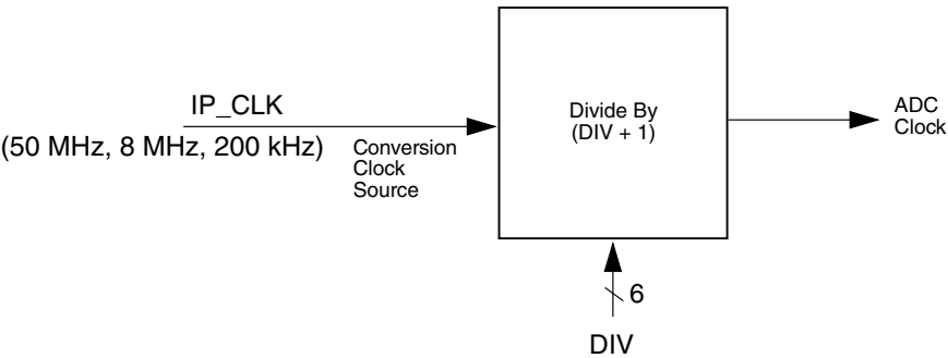
Figure 22-8. ADC Clock Generation
