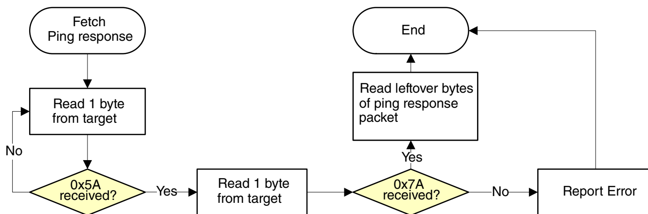
Figure 5-17. Host reads ping response from target via LPI2C
