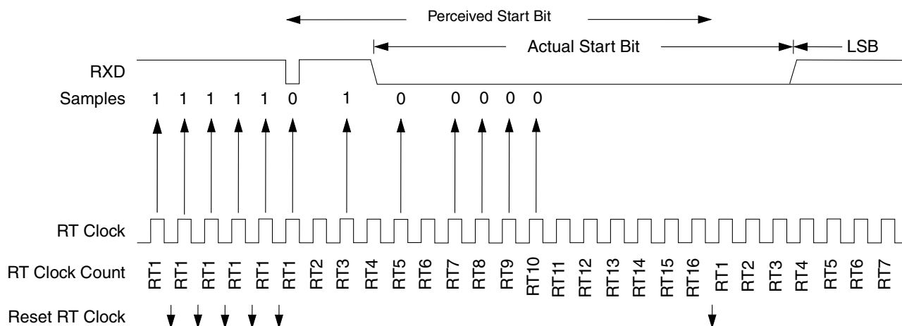
Figure 29-7. Start Bit Search Example 2
