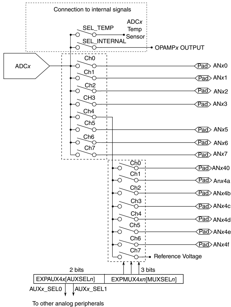
Figure 22-7. Expansion MUX
