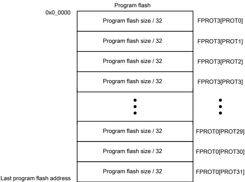
Figure 18-2. Program flash protection
