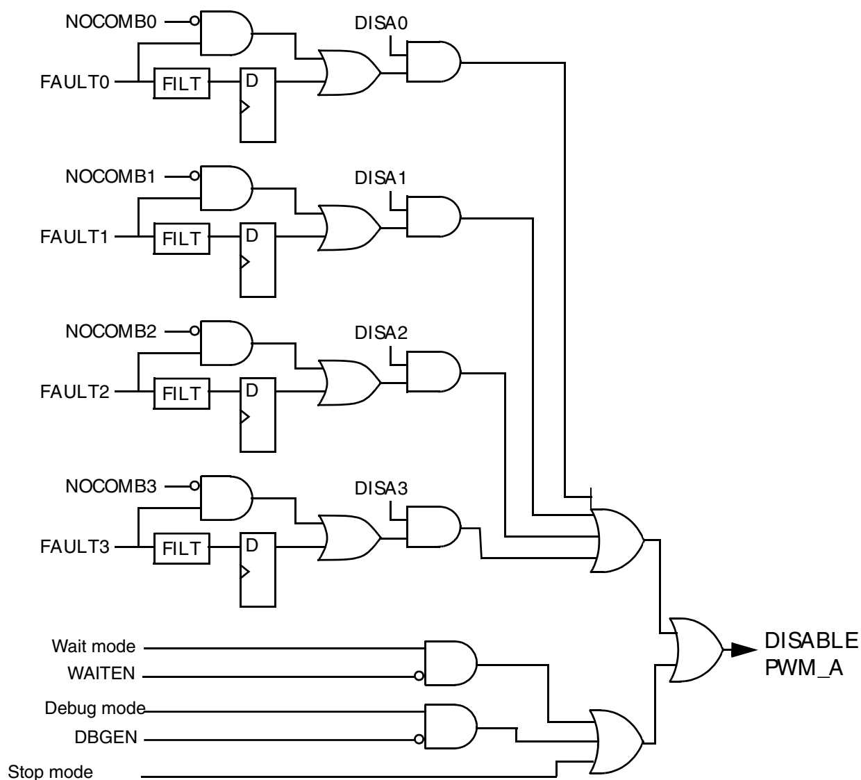
Figure 26-28. Fault decoder for PWM_A
