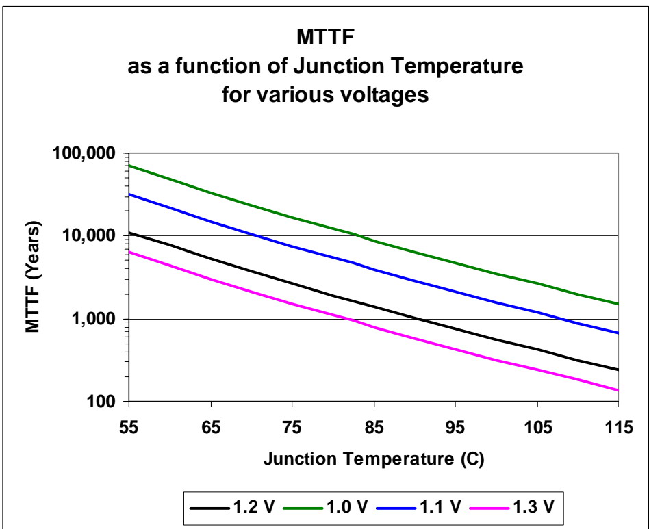
MC7447B FIT Rate and MTTF Derated 60% C.L. Curves.
