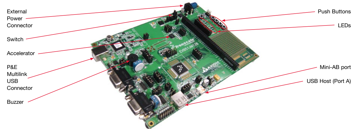
Figure 1. EVB51JM128 board
