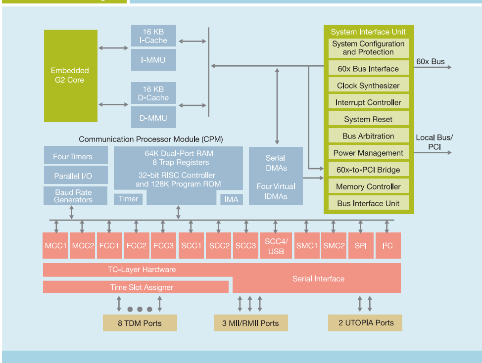
MPC8280 Block Diagram
