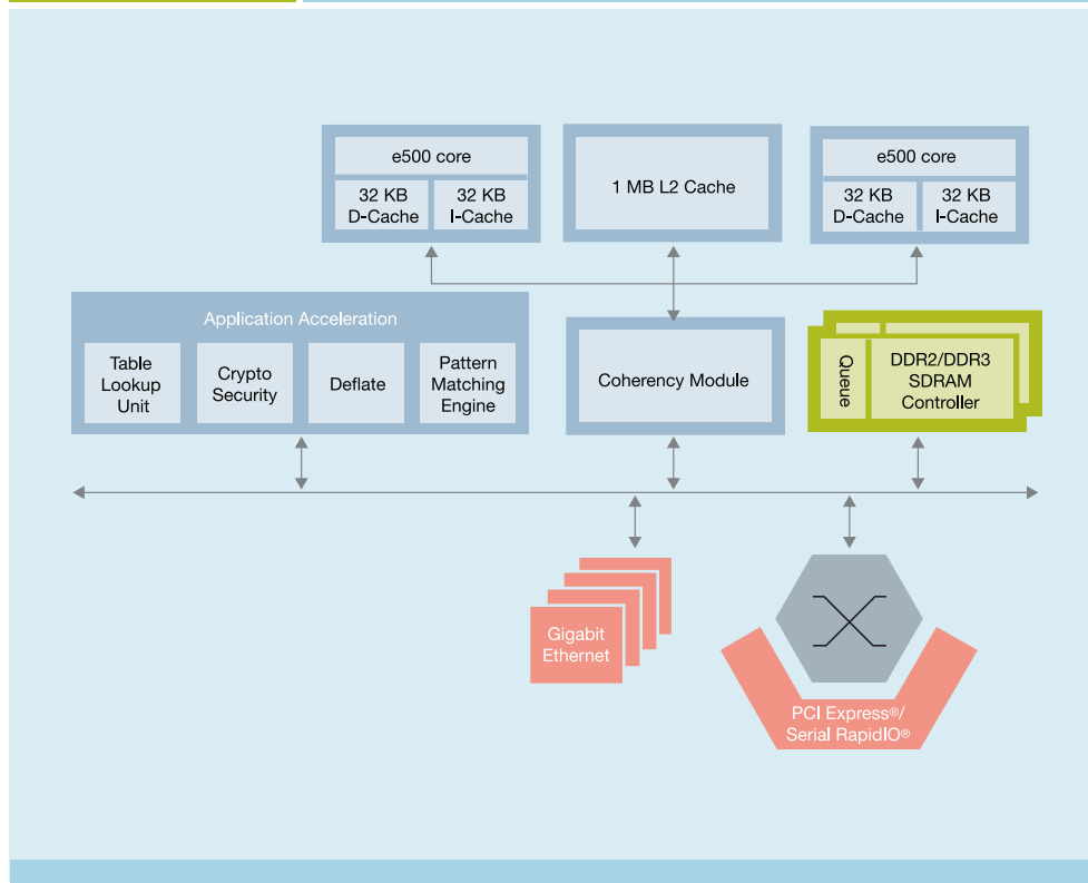
MPC8572 Block Diagram
