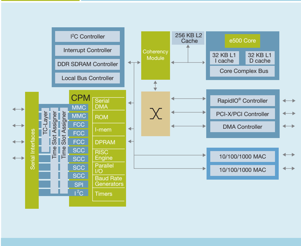
MPC8560 Block Diagram
