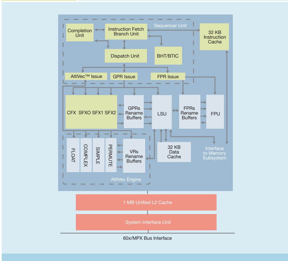
MPC7448 Block Diagram
