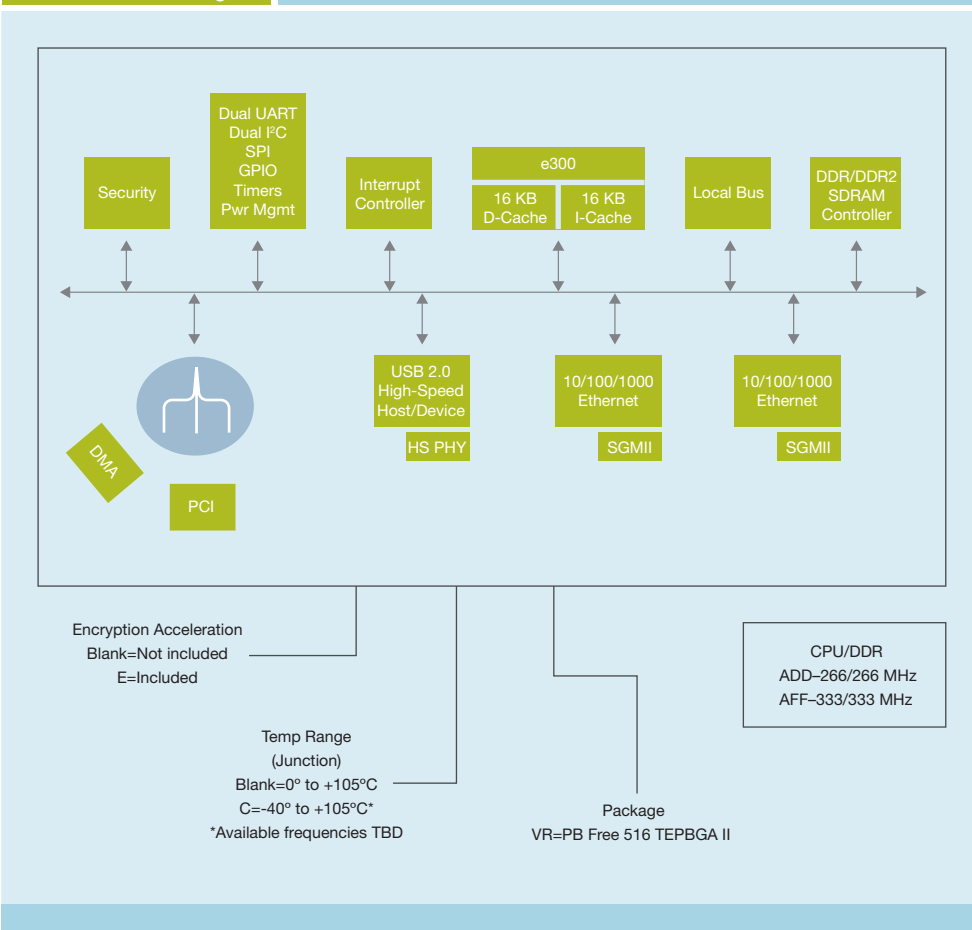
MPC8313E Block Diagram
