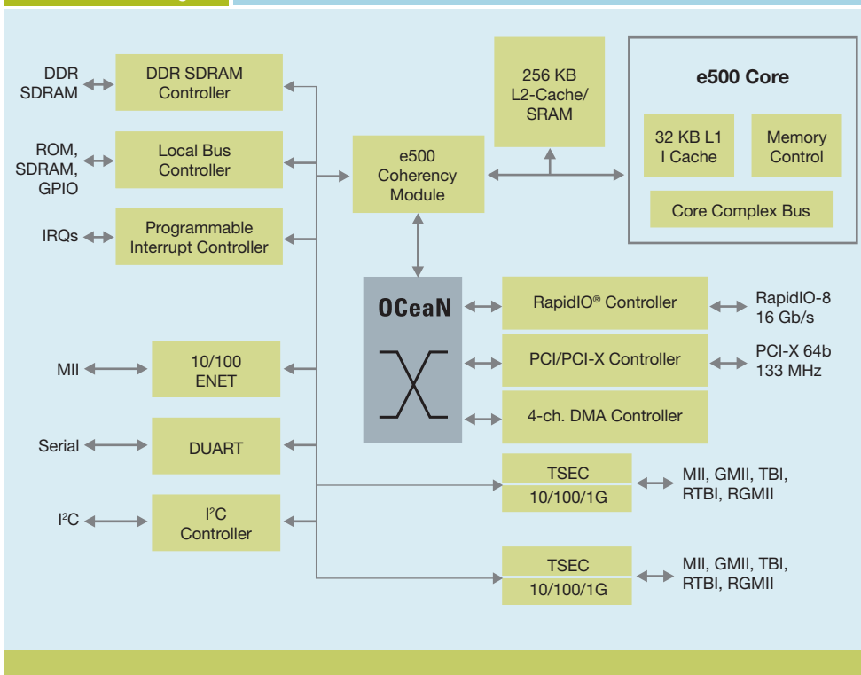
MPC8540 Block Diagram
