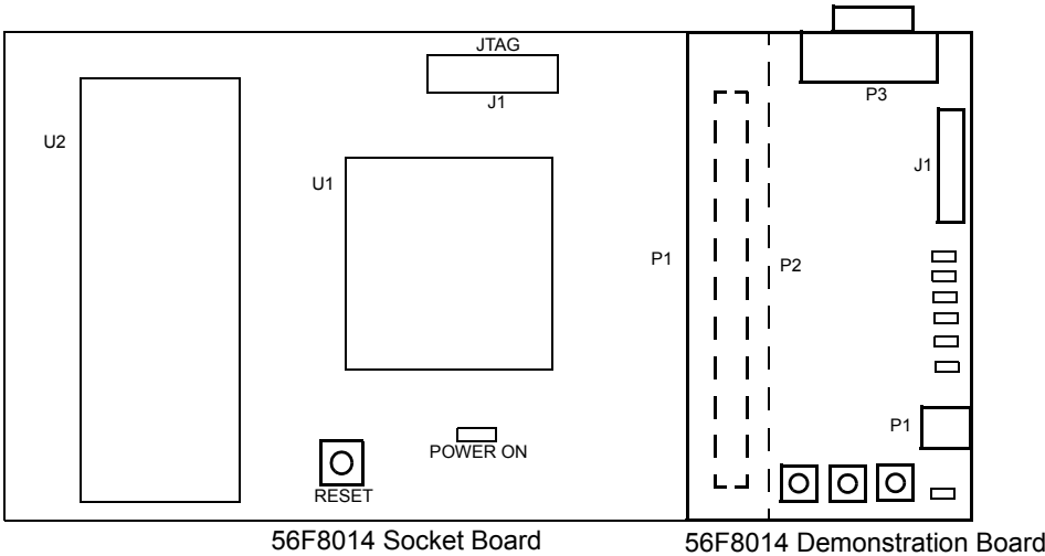
Figure 1-1. Connecting the 56F8014 Socket Board & 56F8014 Demonstration Board
