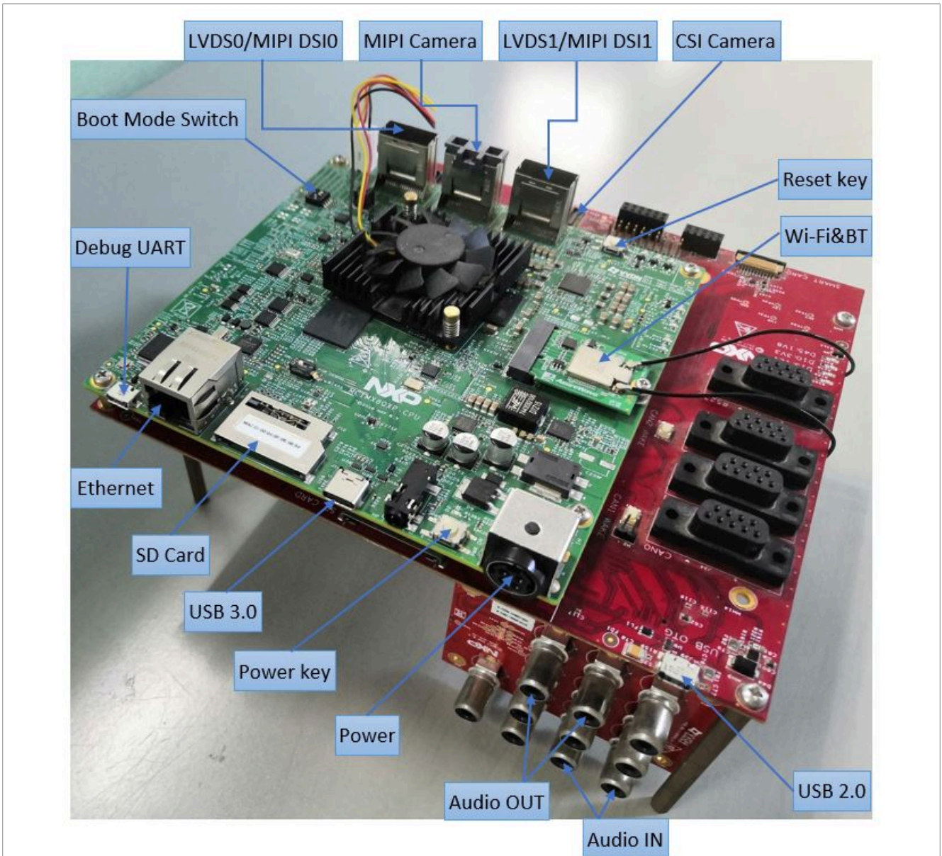
Figure 2. i.MX 8QuadXPlus MEK board
