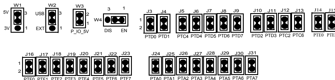
Figure -1 DEMO9S08AW60E Default Settings
