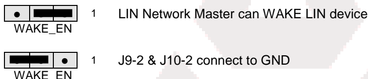
Figure 10: Option Header
