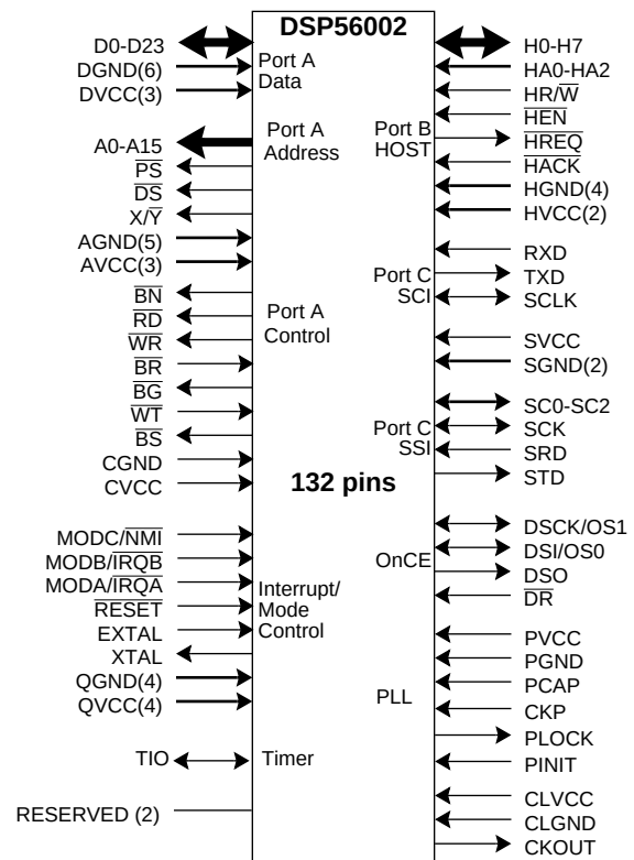
Figure 2-1 DSP56002 Signals
