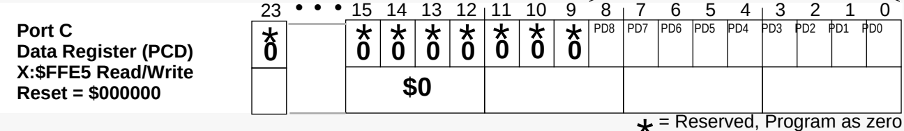
Figure B-12 Port C Data Register (PCD)
