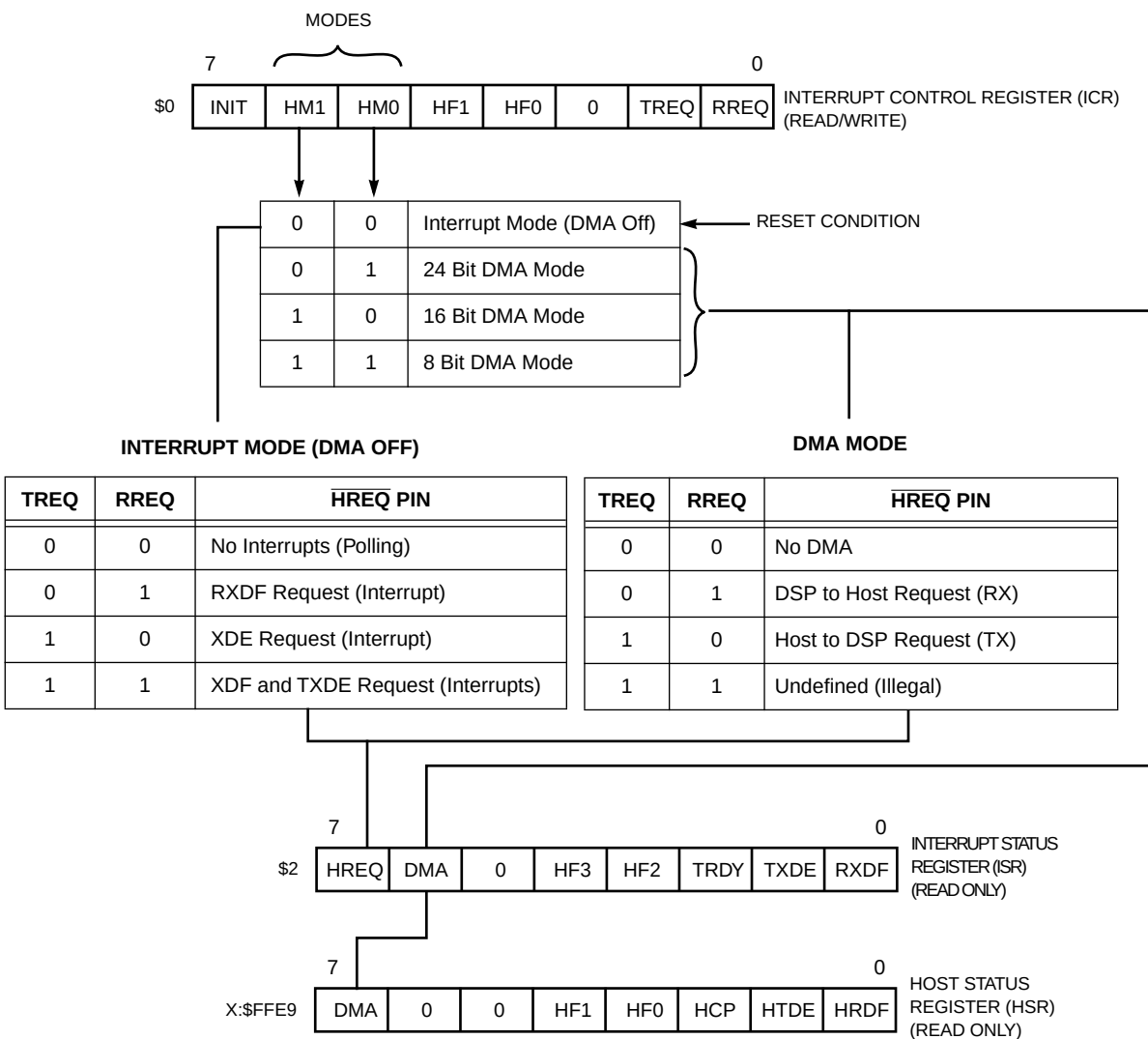
Figure 5-38 Host Bits with TREQ and RREQ
