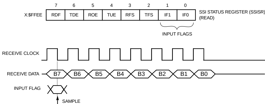
Figure 6-90 Input Flags
