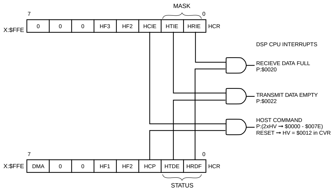
Figure 5-11 HSR-HCR Operation
