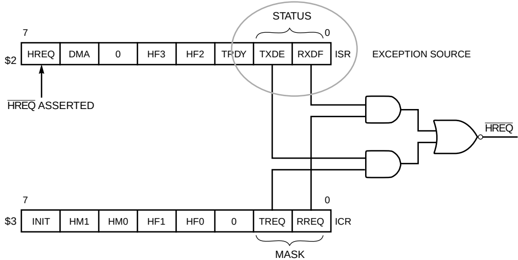
Figure 5-17 HI Interrupt Structure
