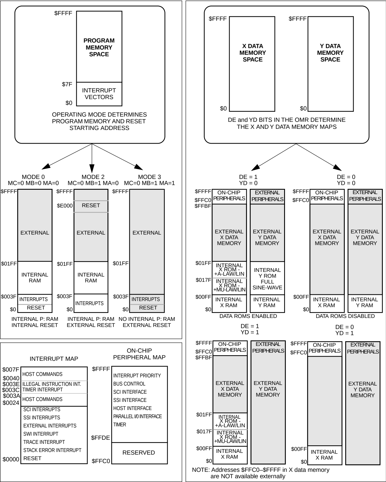
Figure 3-1 DSP56002 Memory Maps
