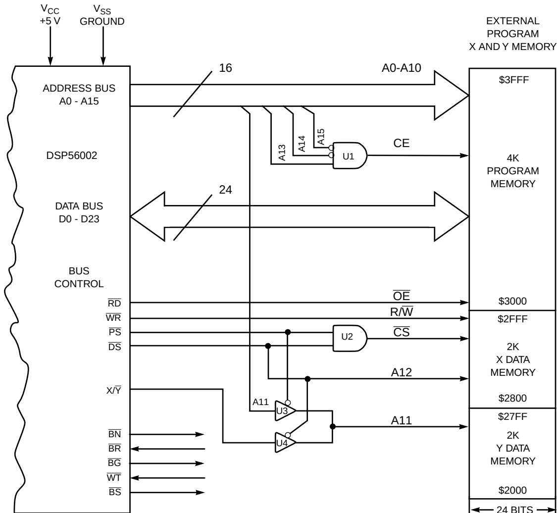
Figure 4-4 Memory Segmentation
