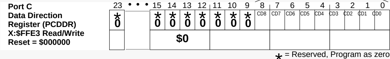
Figure B-11 Port C Data Direction Register (PCDDR)
