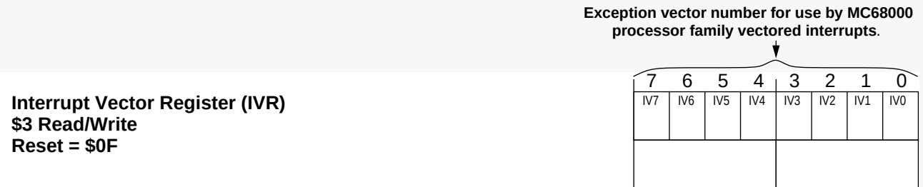
Figure B-21 Interrupt Vector Register (IVR)
