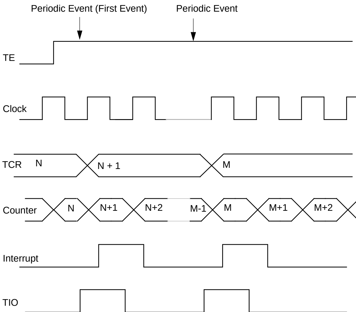
Figure 7-10 Period Measurement Mode (INV=0)
