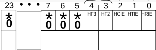
Figure B-14 Host Control Register (HCR)
