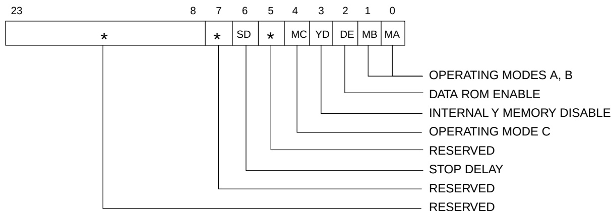
Figure 3-2 OMR Format
