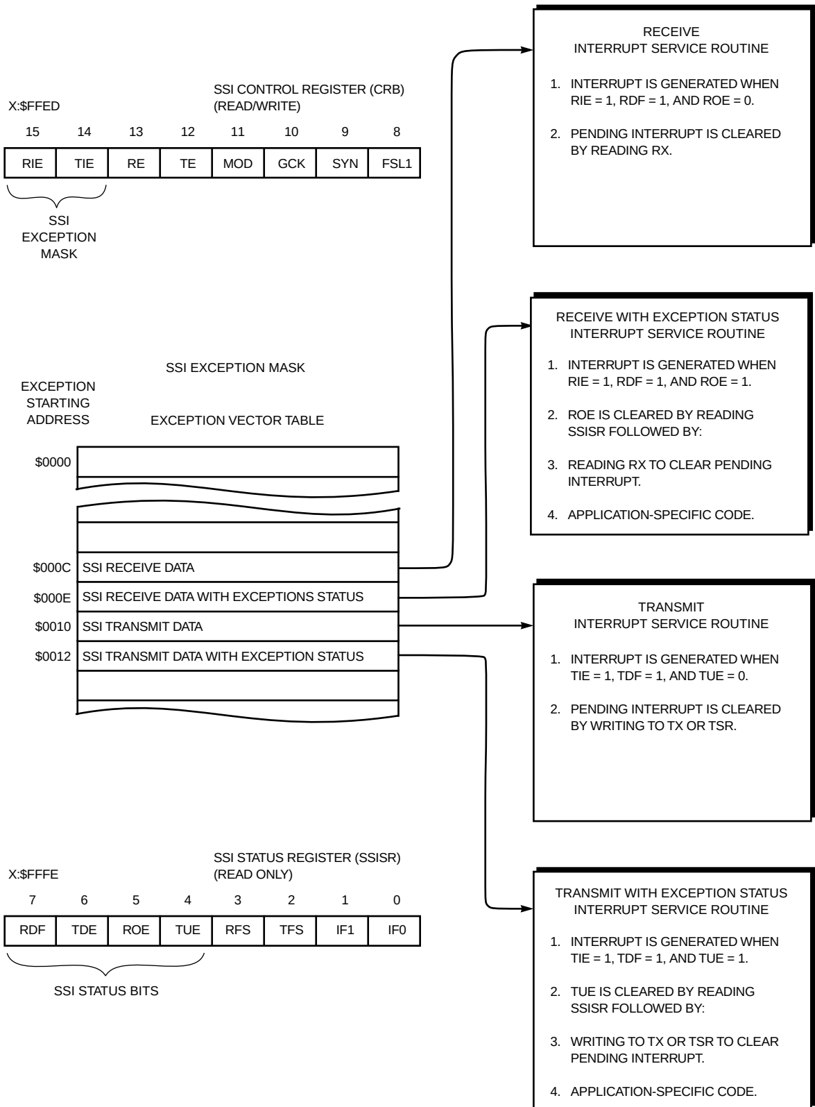
Figure 6-54 SSI Exceptions
