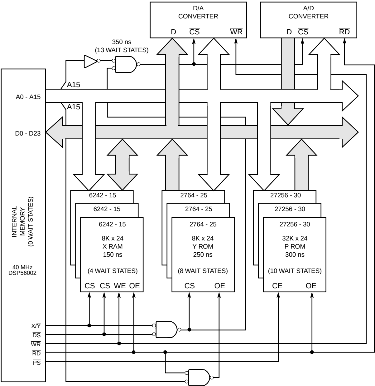
Figure 4-8 Mixed-Speed Expanded System
