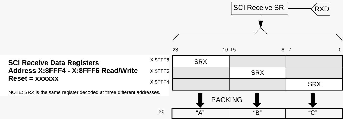
Figure B-29 SCI Receive Data Registers
