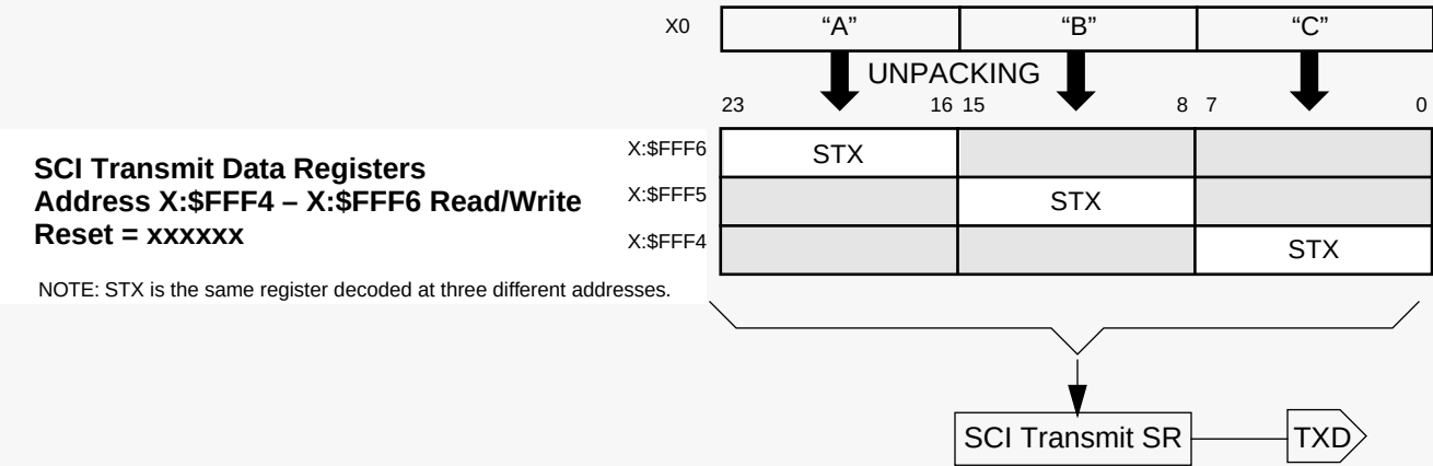
Figure B-28 SCI Transmit Data Registers
