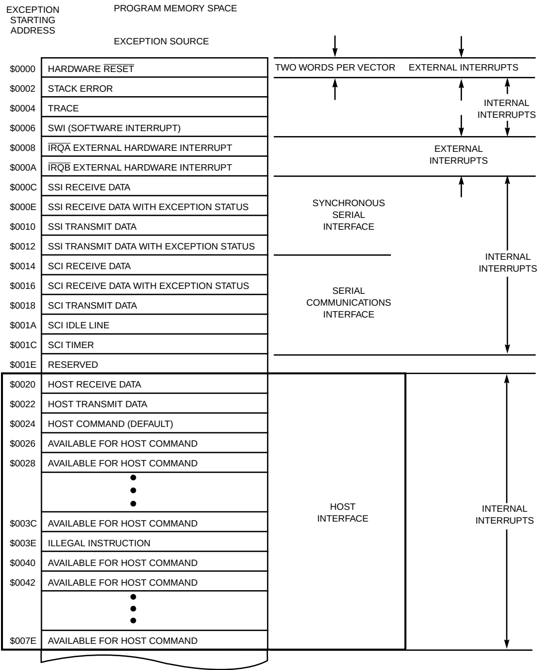
Figure 5-27 HI Exception Vector Locations
