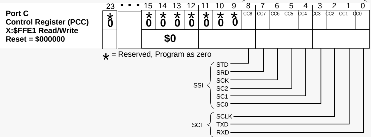
Figure B-10 Port C Control Register (PCC)
