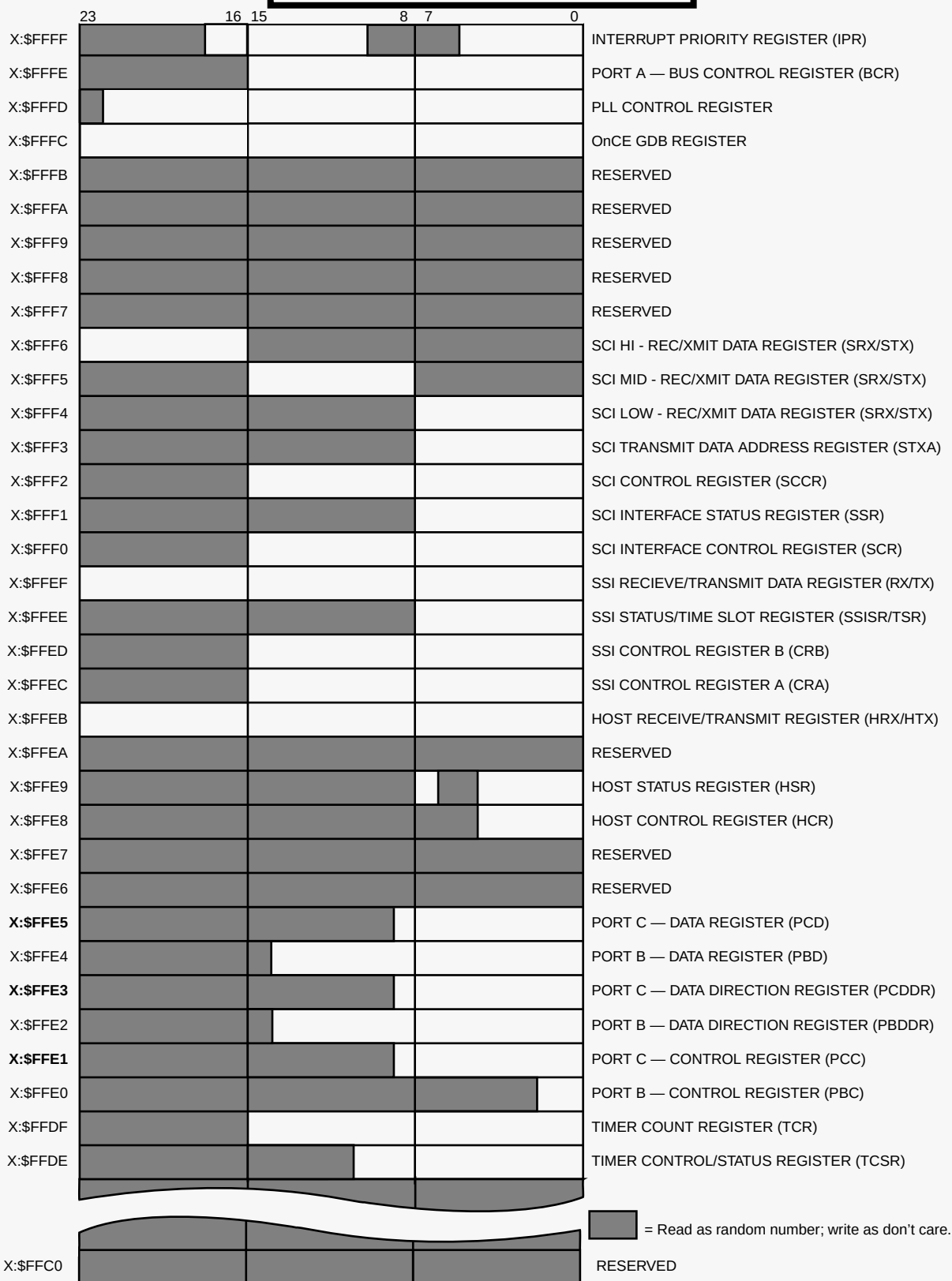
Figure B-1 On-chip Peripheral Memory Map
