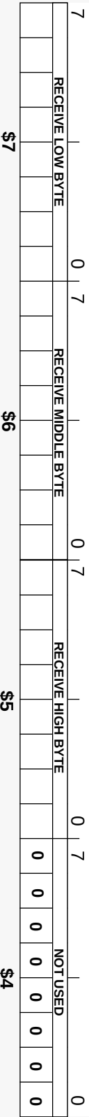
Figure B-22 Receive Byte Registers
