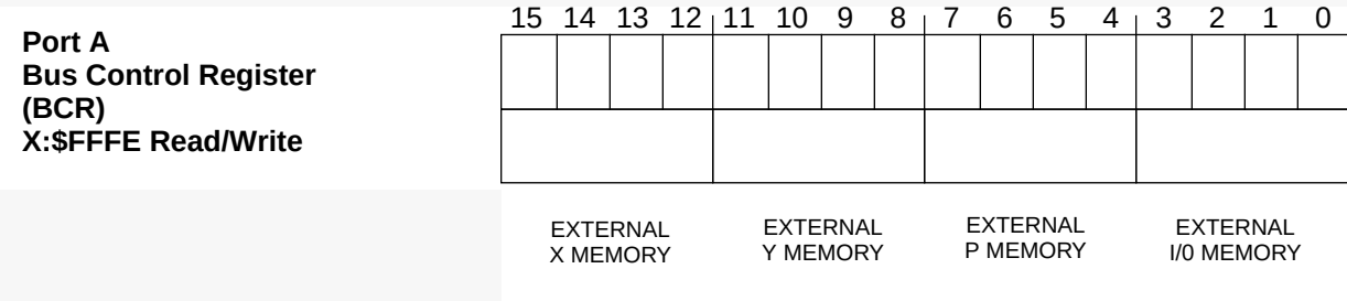
Figure B-3 Bus Control Register (BCR)
