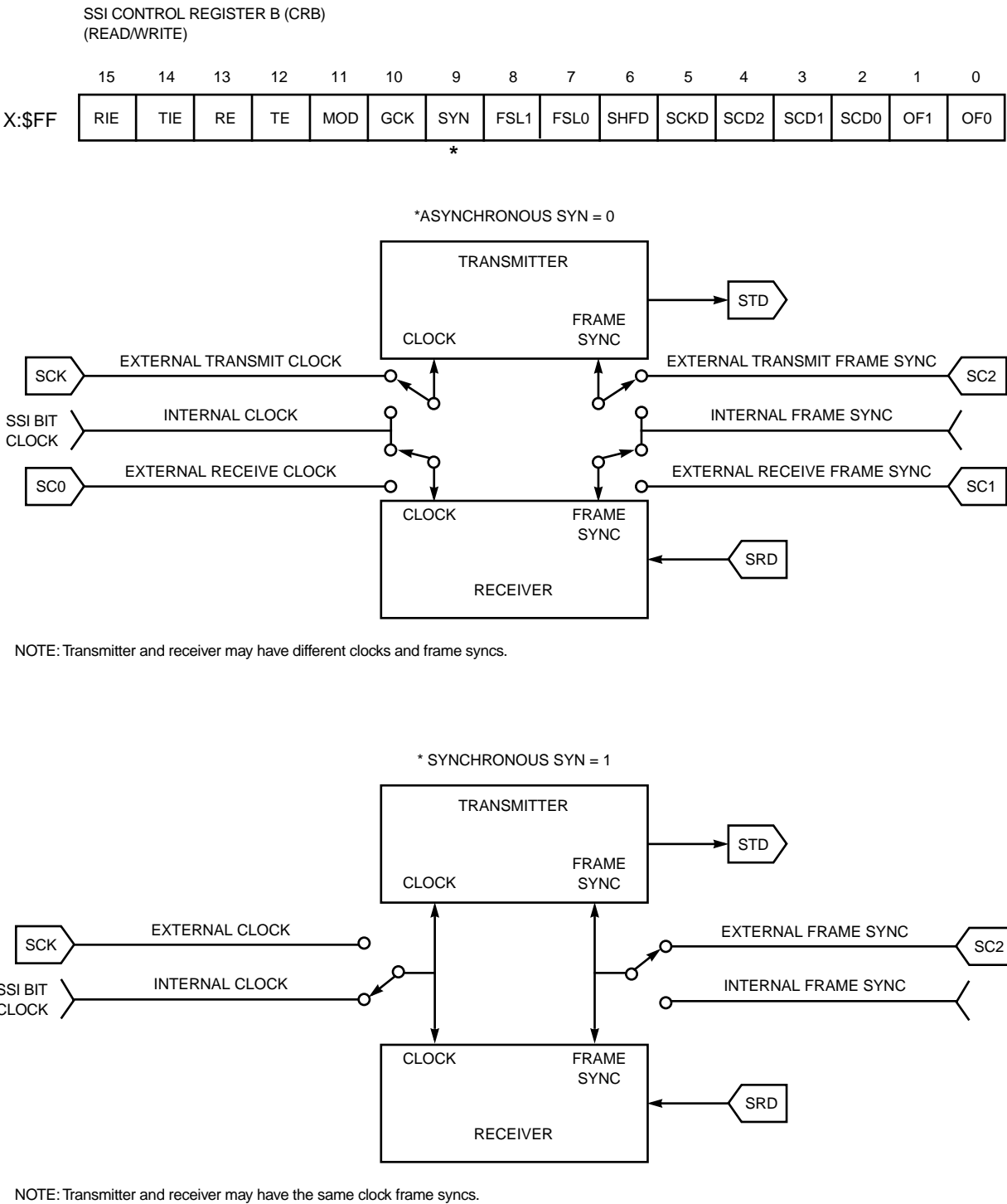
Figure 6-63 CRB SYN Bit Operation
