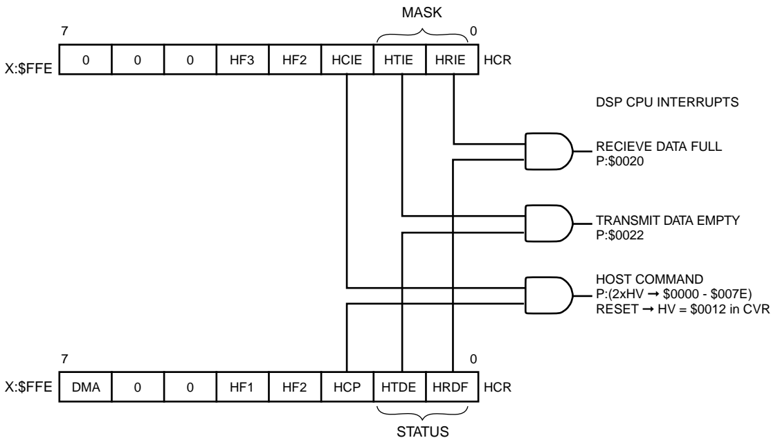
Figure 5-11 HSR-HCR Operation
