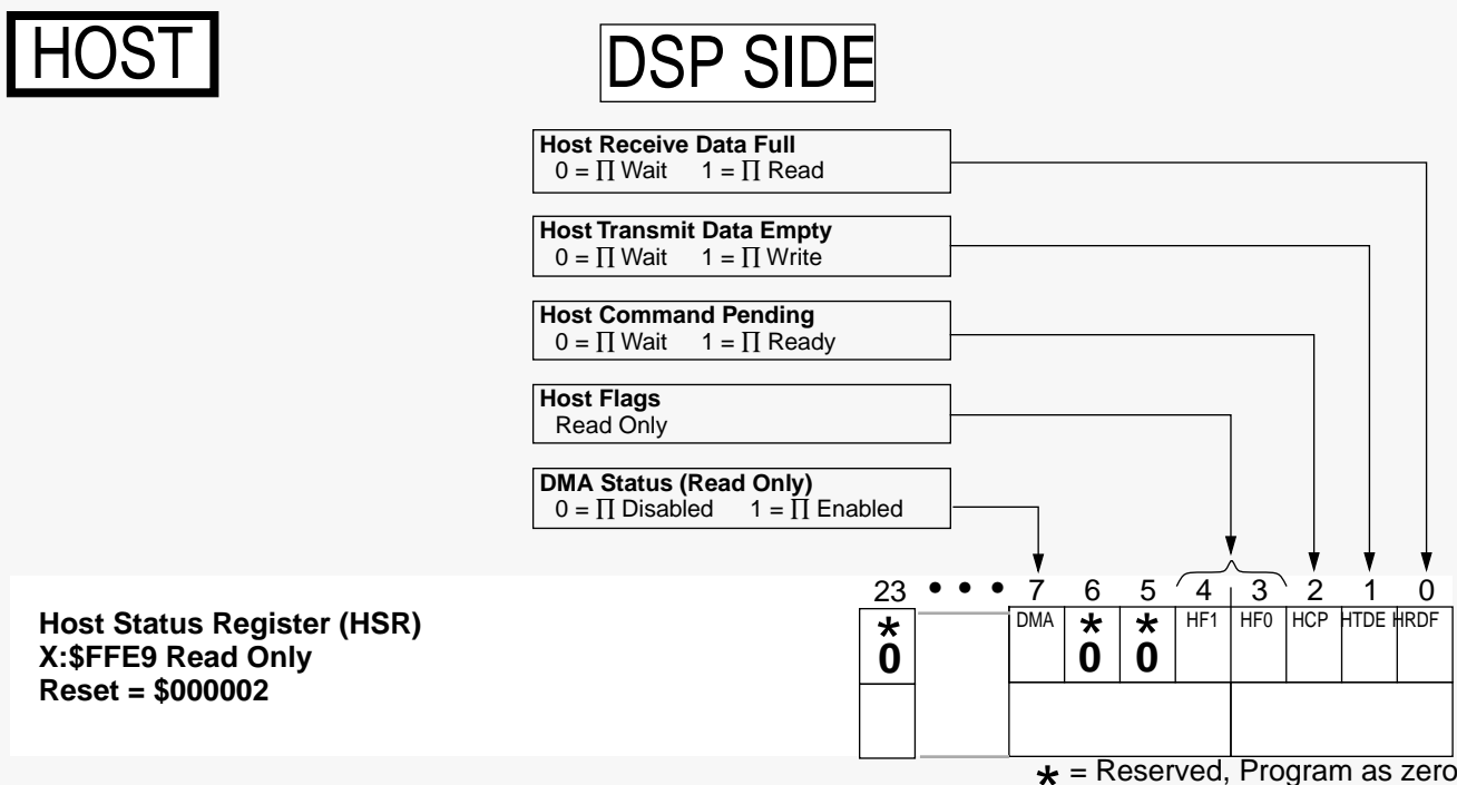
Figure B-15 Host Status Register (HSR)
