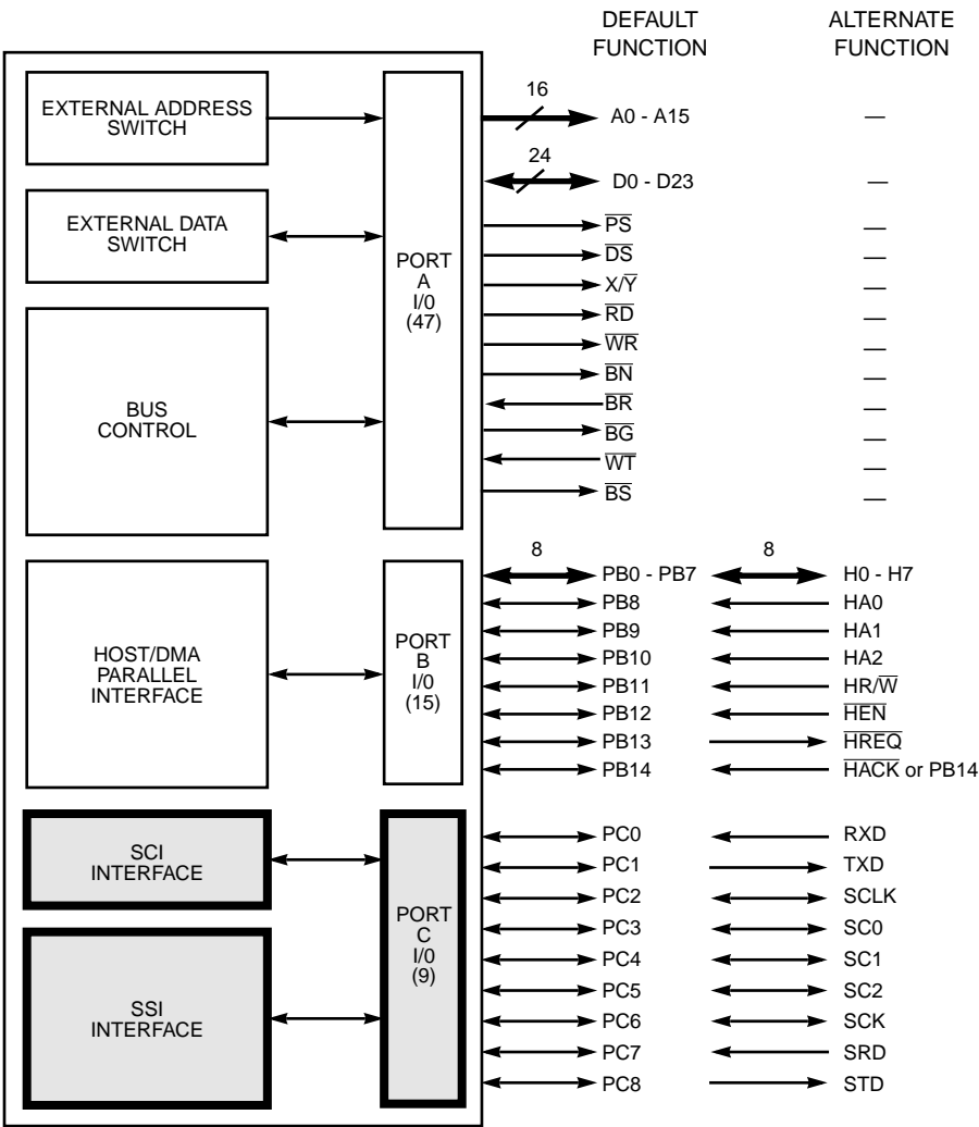
Figure 6-1 Port C Interface
