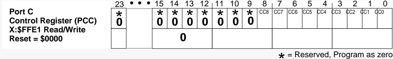
Figure B-30 SSI Control Register (PCC)
