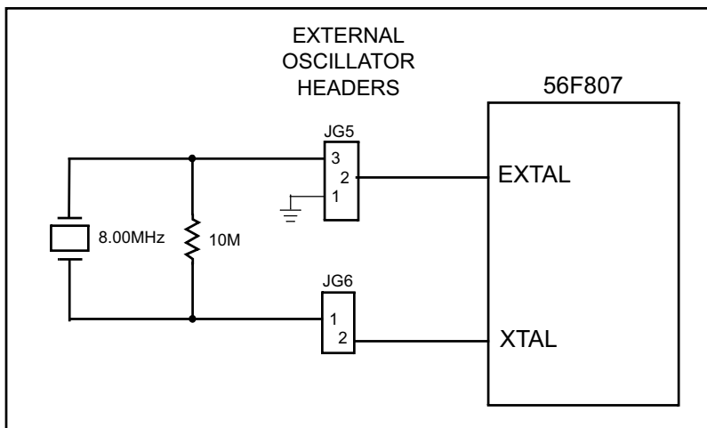
Figure 2-3. Schematic Diagram of the Clock Interface
