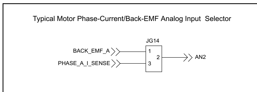
Figure 2-15. Primary Back-EMF or Motor Phase Current Sense Signals
