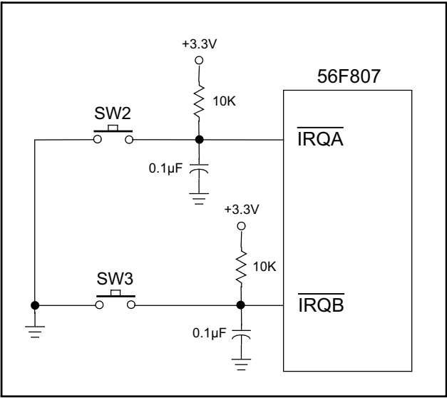
Figure 2-6. Schematic Diagram of the User Interrupt Interface
