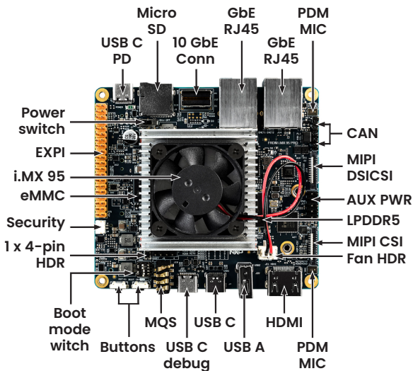
Figure 1: Top view of the FRDM i.MX 95 PRO development board
