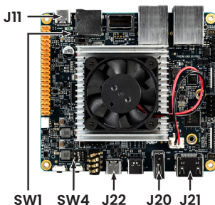
Figure 3: Available connections and switches to get started with the FRDM i.MX 95 PRO development board
