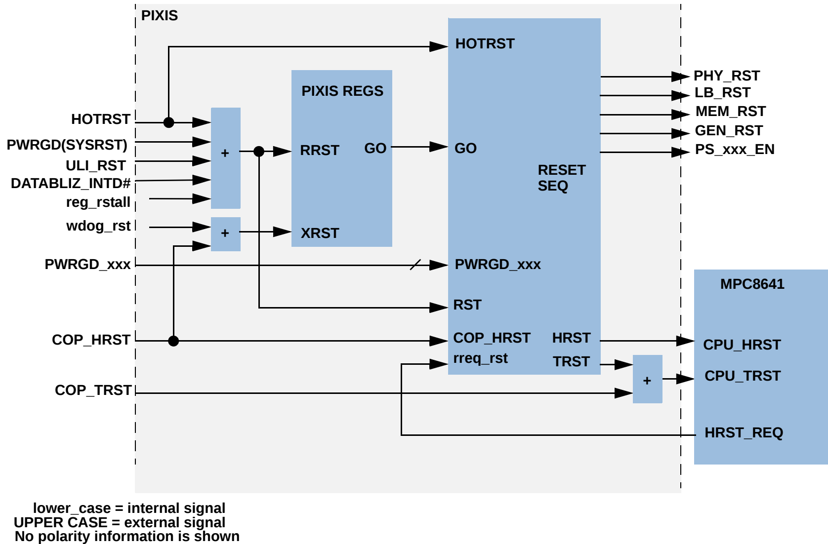
Figure 35. HPCN Reset Hierarchy
