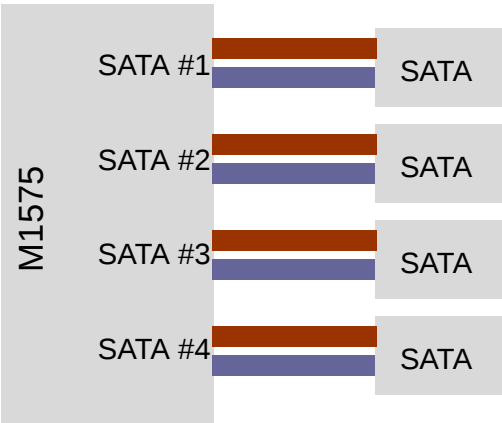
Figure 25. SATA Architecture
