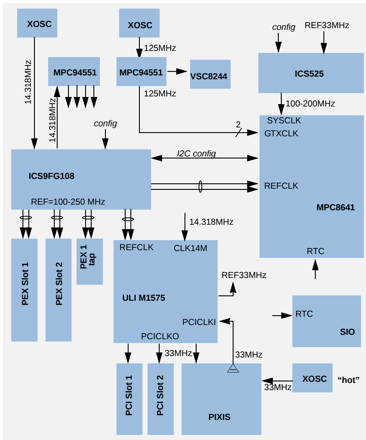
Figure 33. HPCN Clock Architecture
