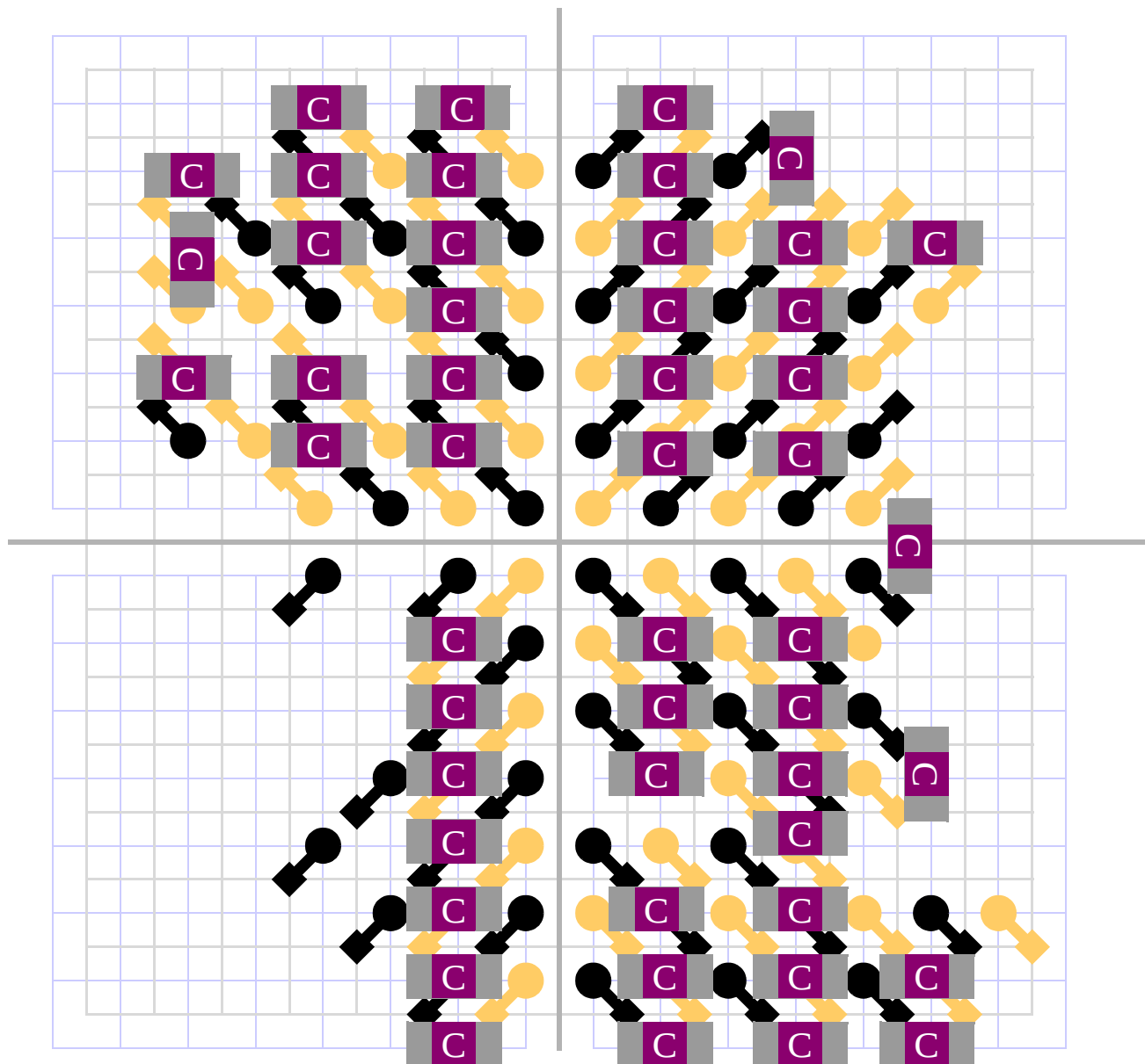
Figure 18. MPC8641 VDD_COREx and Ground SMD 0402 Capacitor Placement
