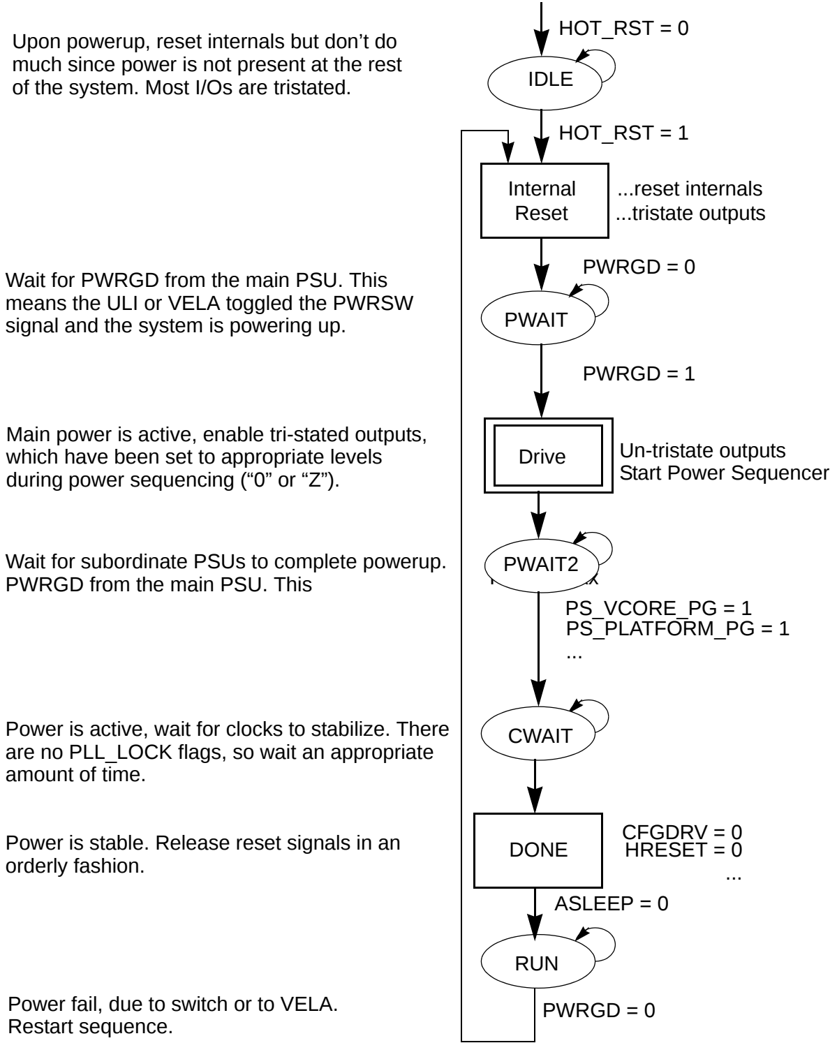
Figure 31. PIXIS Reset Overview
