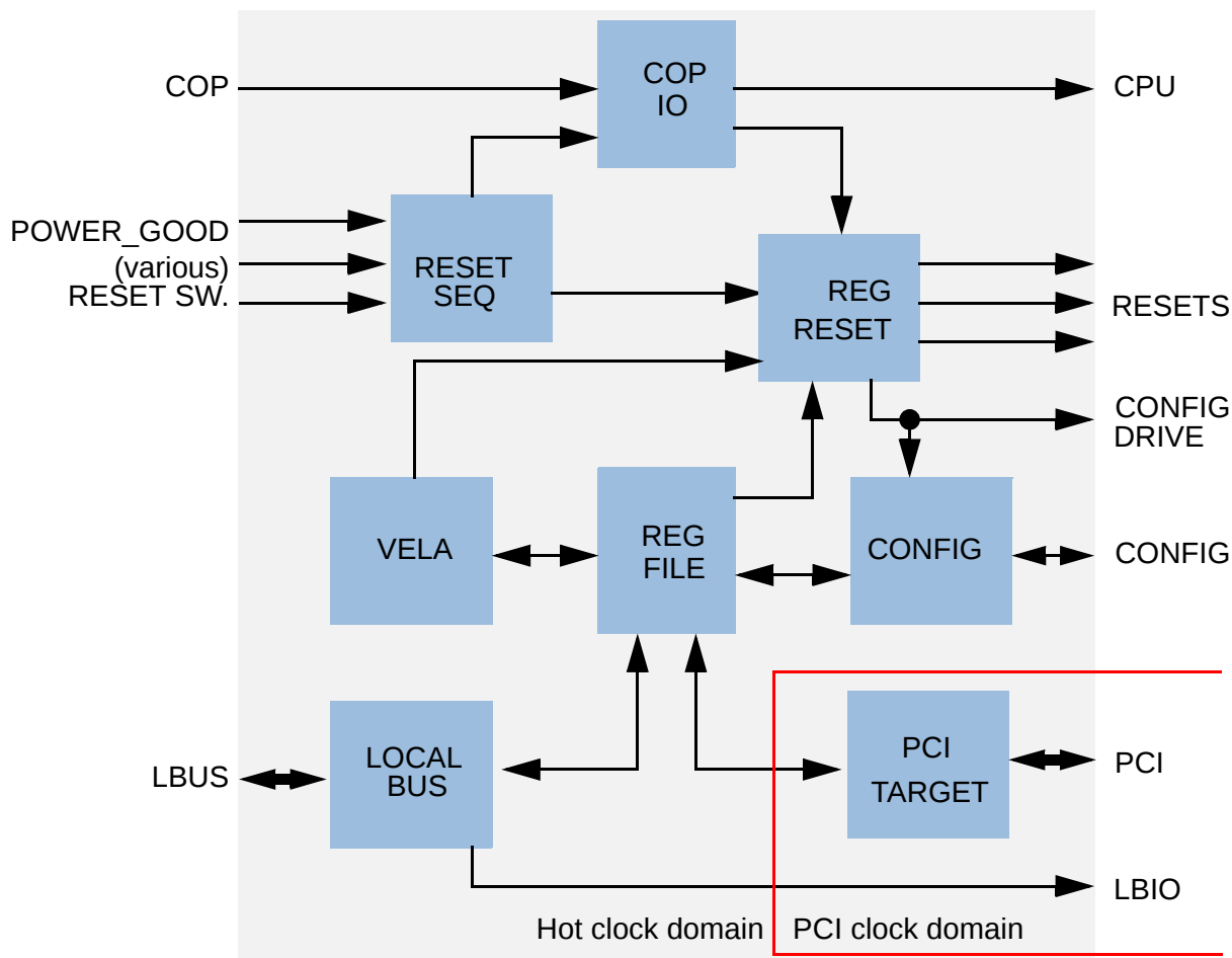
Figure 30. PIXIS Overview
