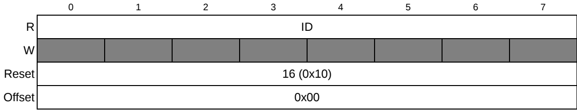
Figure 45. ID Register (PX_ID)
