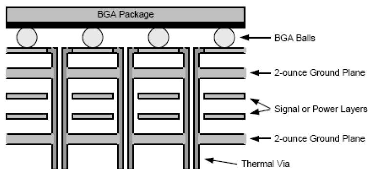
Figure 9: Thermal Ground Plane Connections
