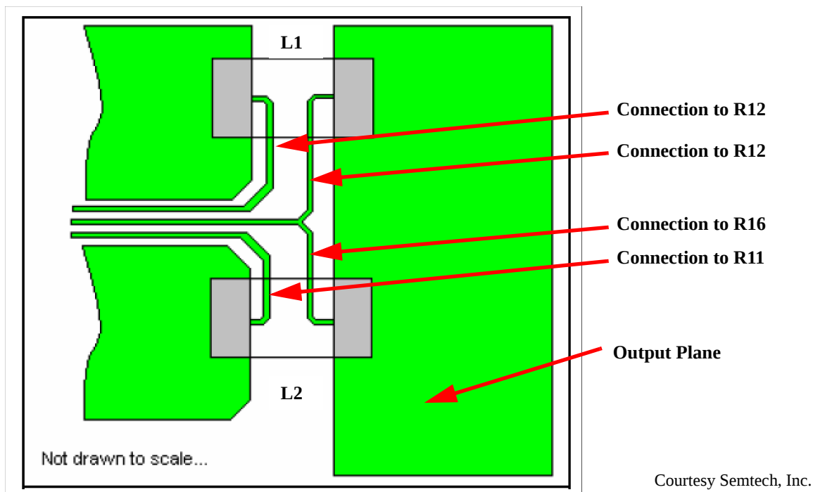
Figure 43. SC458 Kelvin Connection
