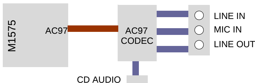
Figure 29. Audio Architecture
