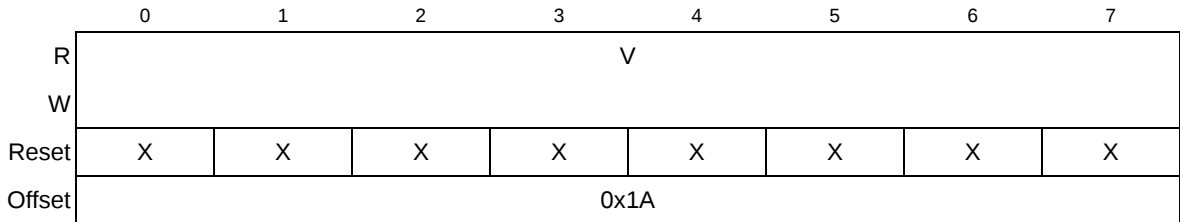
Figure 62. VELA VCLKL Register (PX_VCLKL)
