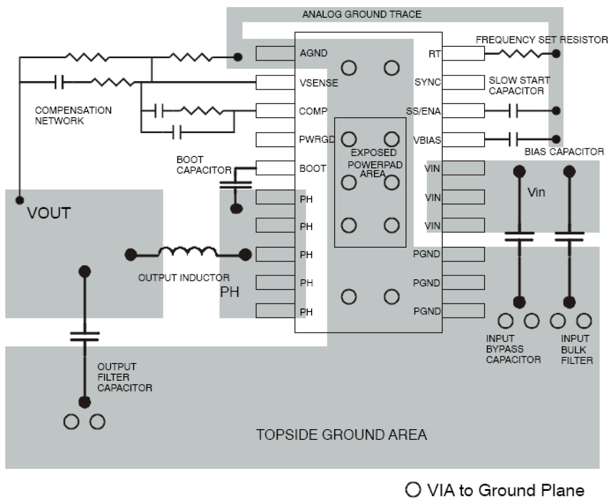
Figure 42. TPS54310 Suggested Layout
