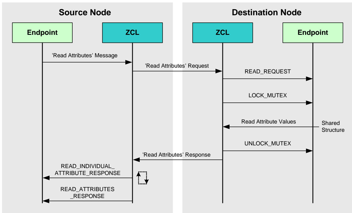
Figure 3: 'Read Attributes' Request and Response
