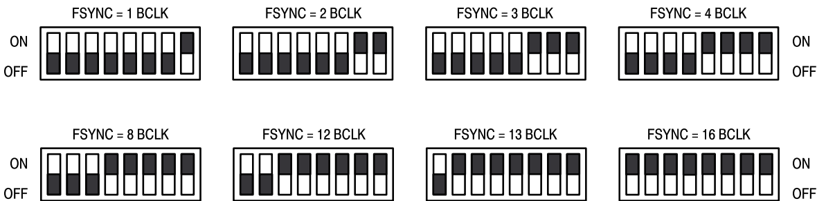
Figure 2–1. Switch S1 Settings for FSYNC Duration
